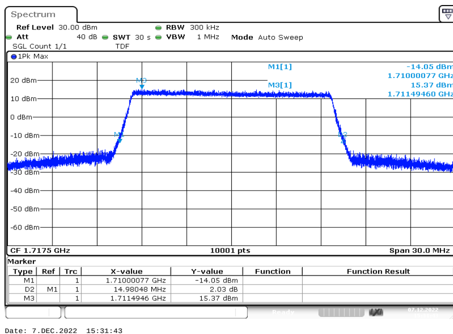
Plot 98: 15 MHz – 16-QAM - lowest channel (-26 dBc BW)
