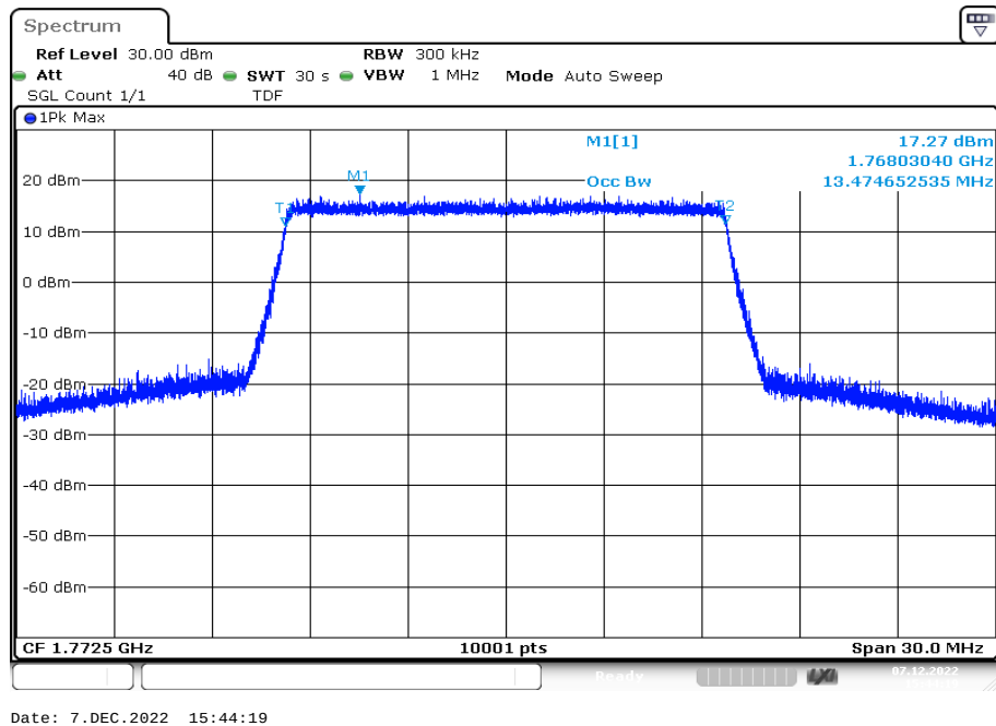
Plot 29: 15 MHz – QPSK - highest channel (99% - OBW)
