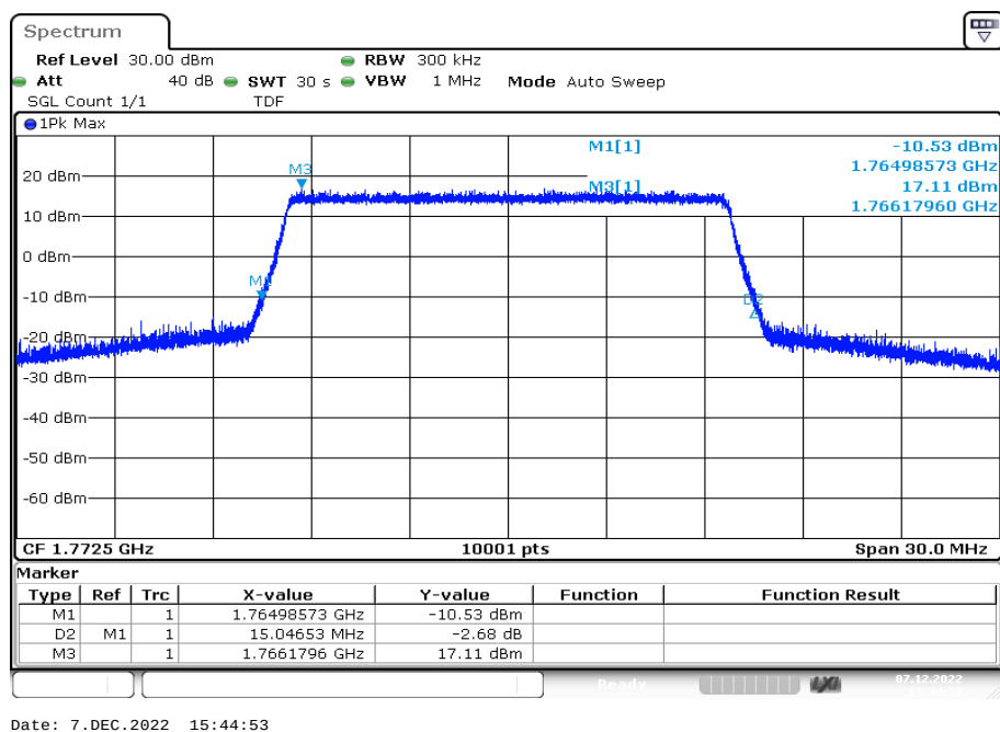
Plot 30: 15 MHz – QPSK - highest channel (-26 dBc BW)
