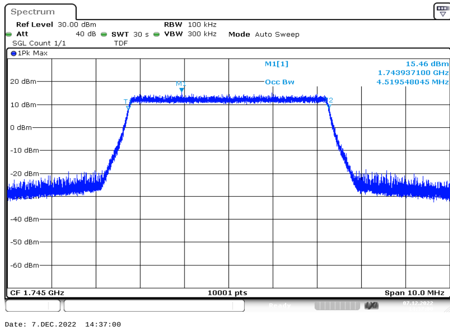
Plot 87: 5 MHz – 64-QAM - middle channel (99% - OBW)
