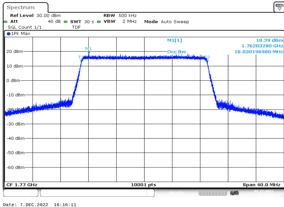
Plot 35: 20 MHz – QPSK - highest channel (99% - OBW)
