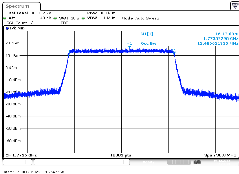
Plot 65: 15 MHz – 16-QAM - highest channel (99% - OBW)
