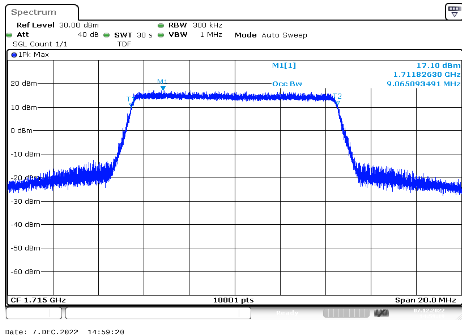
Plot 91: 10 MHz – 64-QAM - lowest channel (99% - OBW)
