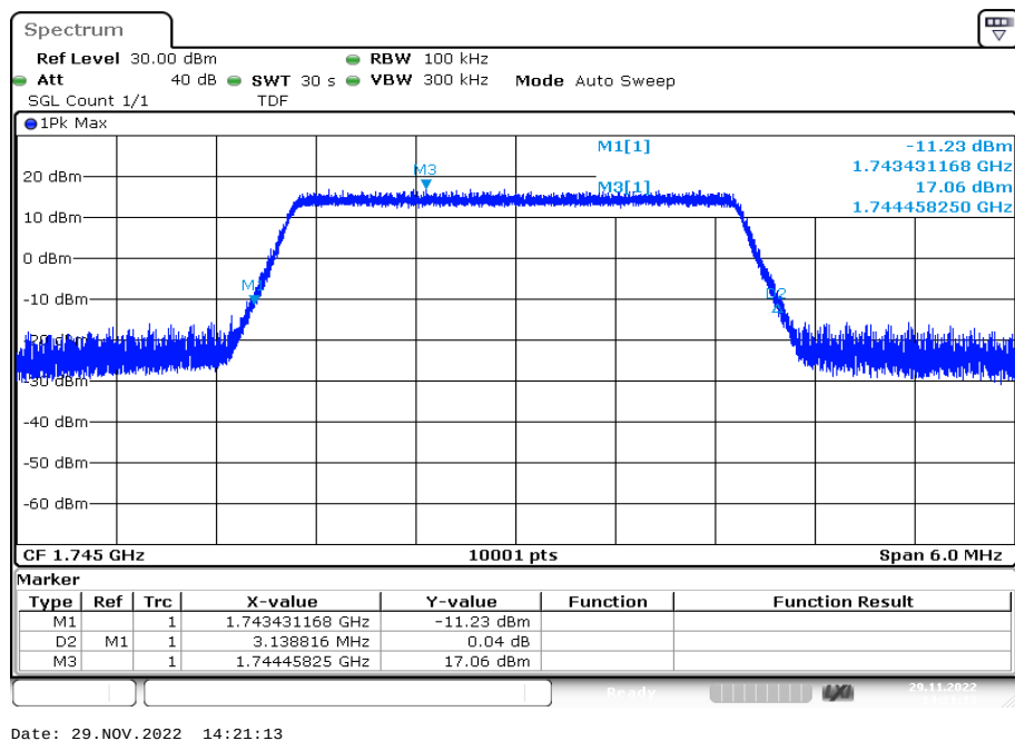
Plot 82: 3 MHz – 64-QAM - middle channel (-26 dBc BW)
