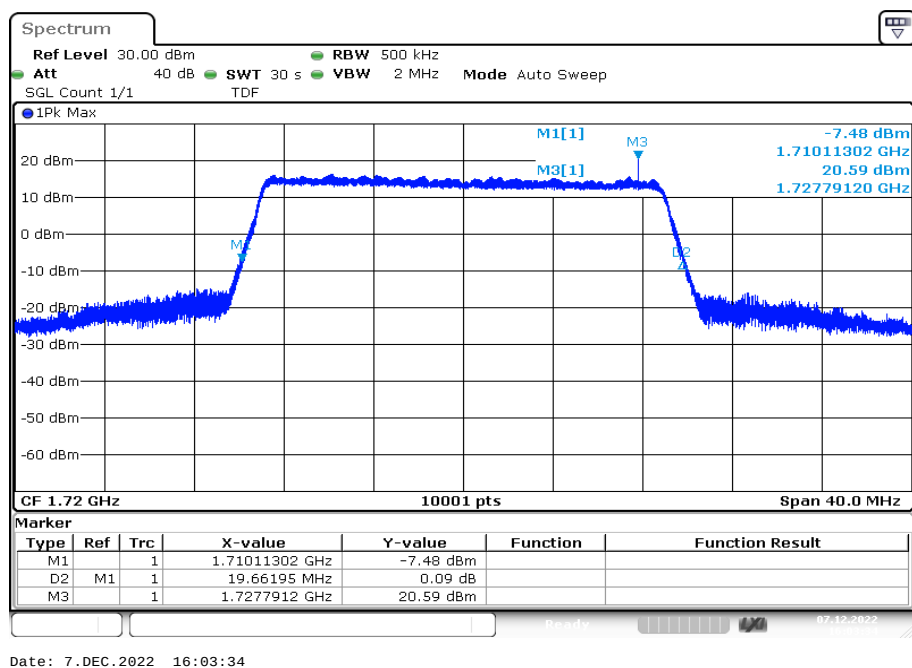
Plot 104: 20 MHz – 64-QAM - lowest channel (-26 dBc BW)
