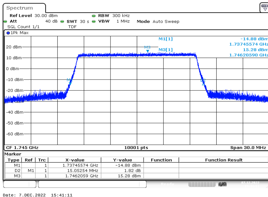
Plot 100: 15 MHz – 64-QAM - middle channel (-26 dBc BW)
