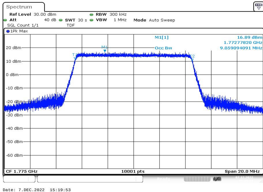
Plot 95: 10 MHz – 64-QAM - highest channel (99% - OBW)
