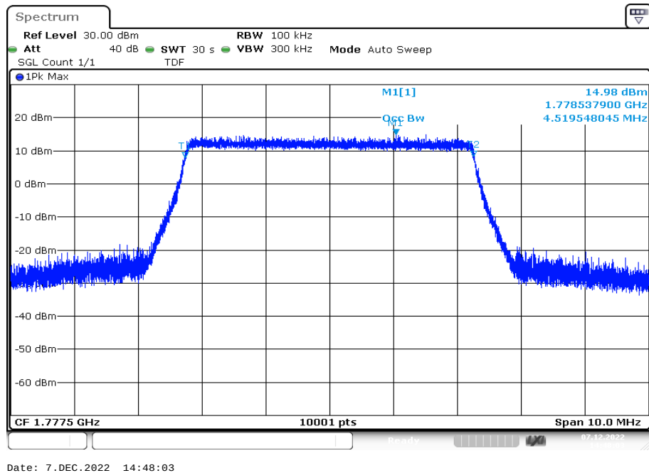
Plot 89: 5 MHz – 64-QAM - highest channel (99% - OBW)
