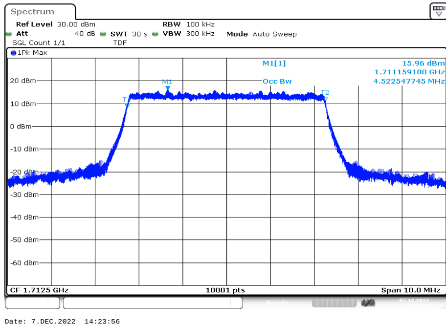
Plot 49: 5 MHz – 16-QAM - lowest channel (99% - OBW)
