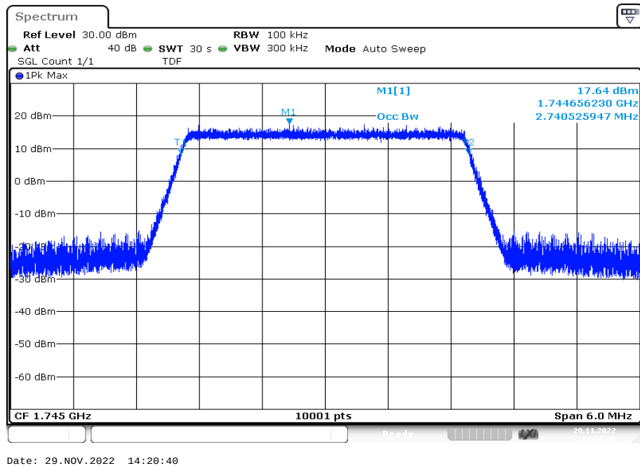
Plot 81: 3 MHz – 64-QAM - middle channel (99% - OBW)
