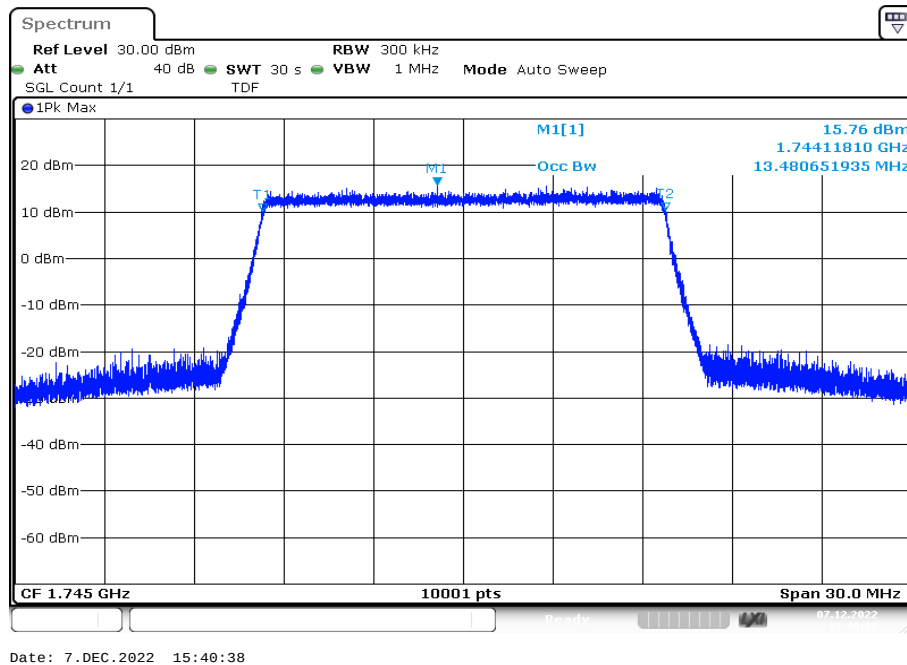
Plot 99: 15 MHz – 64-QAM - middle channel (99% - OBW)
