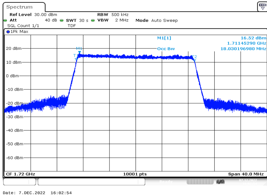
Plot 103: 20 MHz – 64-QAM - lowest channel (99% - OBW)
