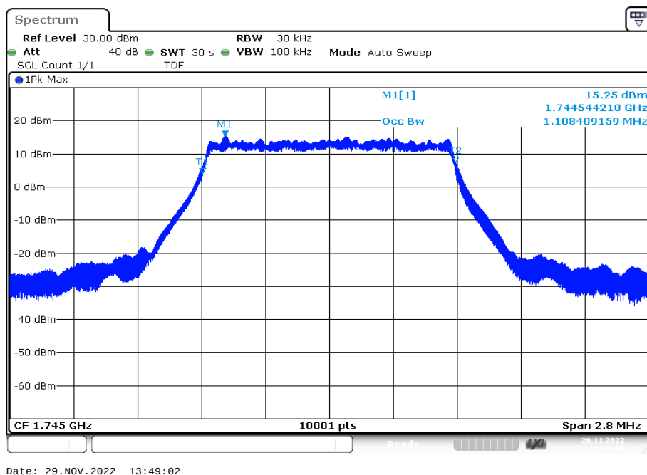
Plot 75: 1.4 MHz – 64-QAM - middle channel (99% - OBW)
