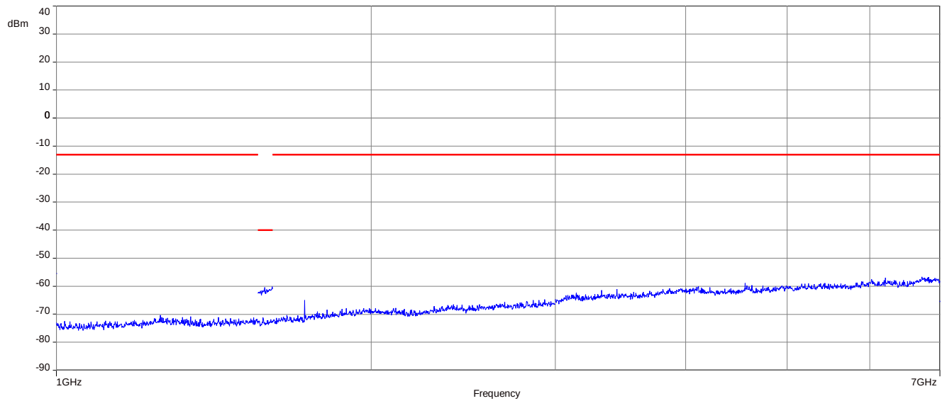
Plot 6: 16-QAM - Middle channel (1 GHz – 7 GHz)
