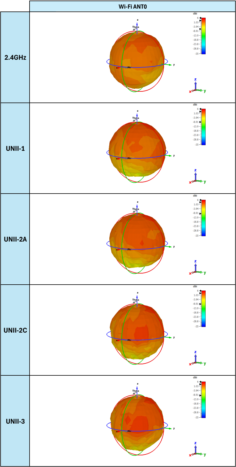
The above plots represent radiation patterns, obtained by combining all antennas in accordance with the methodology defined in FCC KDB 662911 D01 v02r01, Section F.2.d.i, and evaluated over the full spherical surface enclosing the equipment under test. Each Pattern corresponds to the maximum radiation pattern between both polarization at a specific frequency range.
