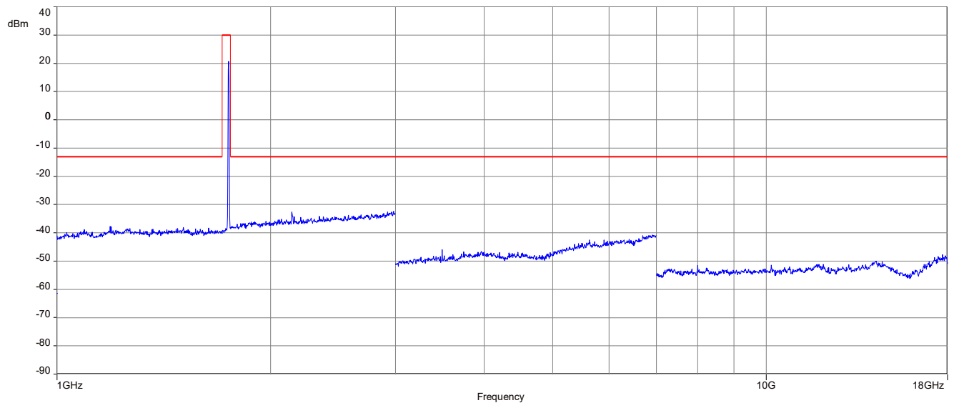
Plot 12: Middle channel (1 GHz – 18 GHz), LTE band 66
