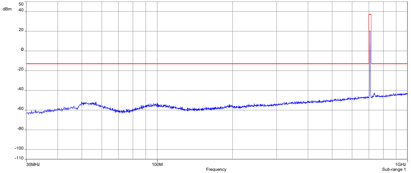
Plot 7: Middle channel (30 MHz – 1 GHz), LTE band 12
