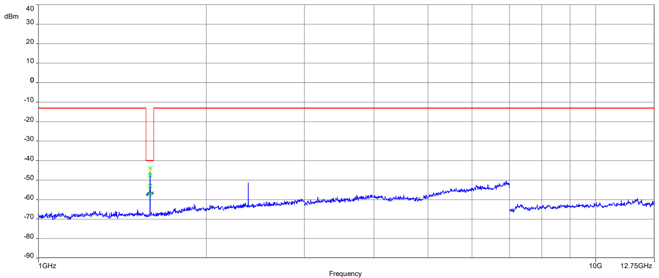
Plot 10: Middle channel (1 GHz – 12.75 GHz), LTE band 14
