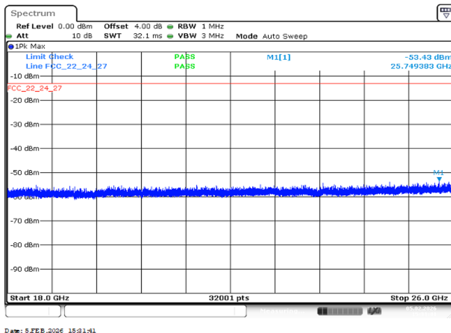
Plot 4: Middle channel (18 GHz – 26 GHz) , LTE band 2
