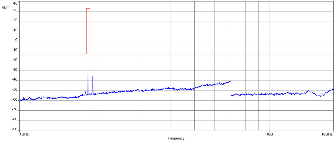
Plot 3: Middle channel (1 GHz – 18 GHz) , LTE band 2
