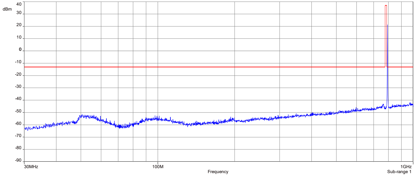
Plot 9: Middle channel (30 MHz – 1 GHz), LTE band 14
