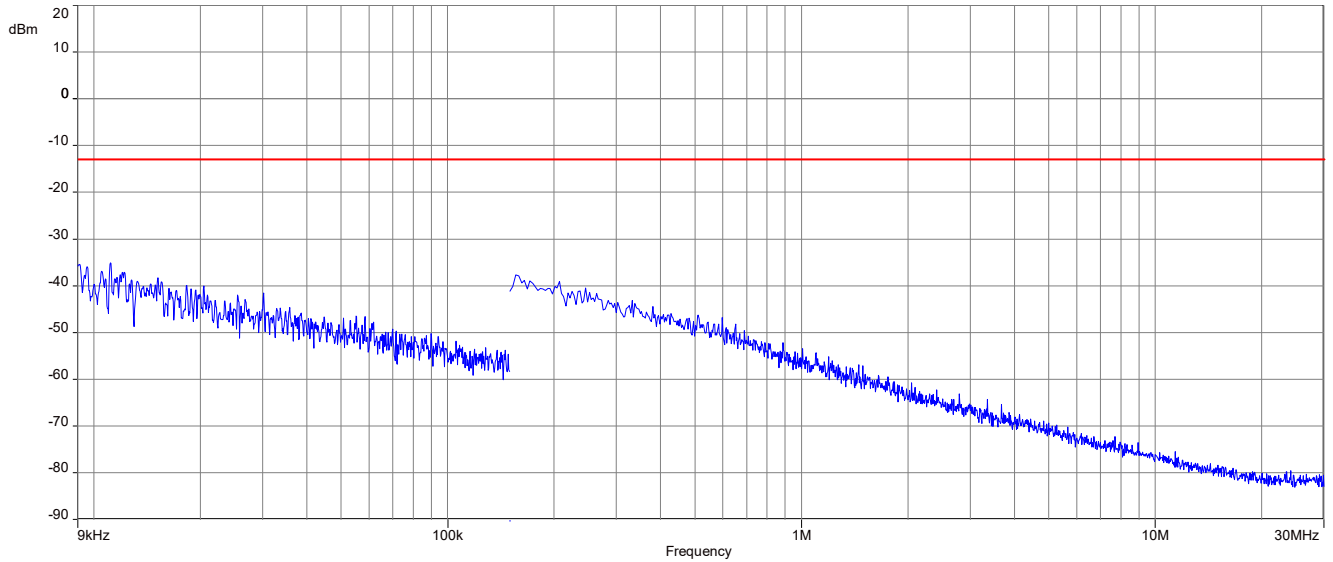
Plot 1: Middle channel (9 kHz - 30 MHz), worst case for all LTE bands
