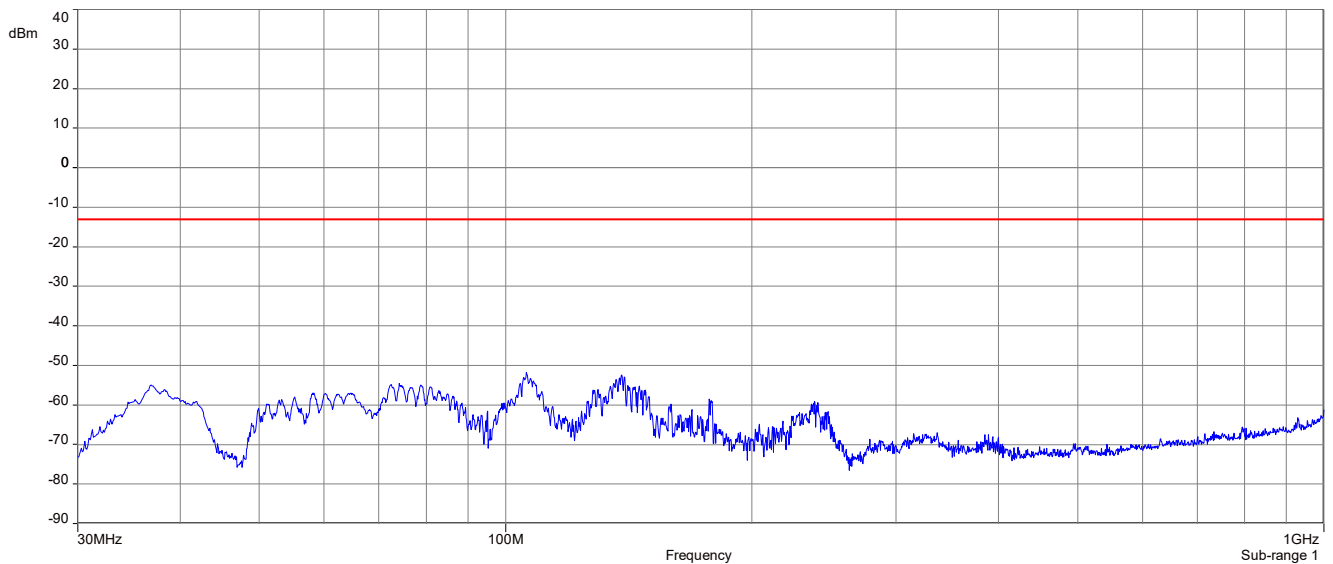
Plot 2: Middle channel (30 MHz – 1 GHz), LTE band 2
