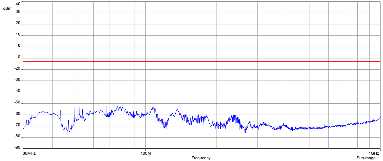
Plot 11: Middle channel (30 MHz – 1 GHz), LTE band 66
