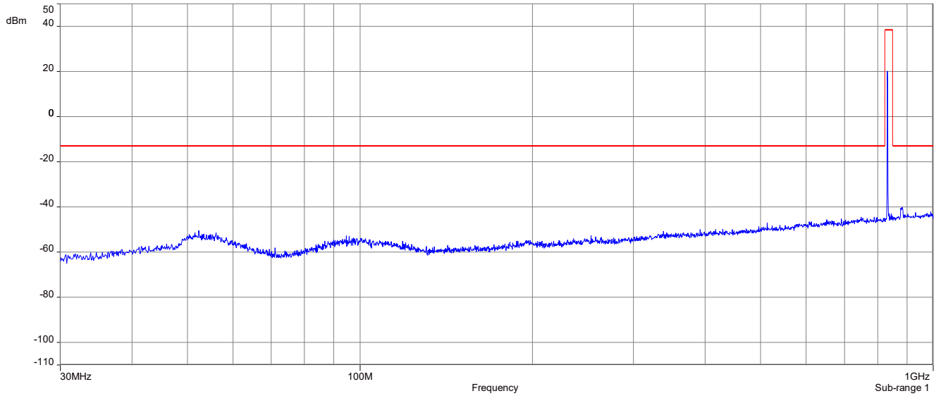
Plot 5: Middle channel (30 MHz – 1 GHz), LTE band 5
