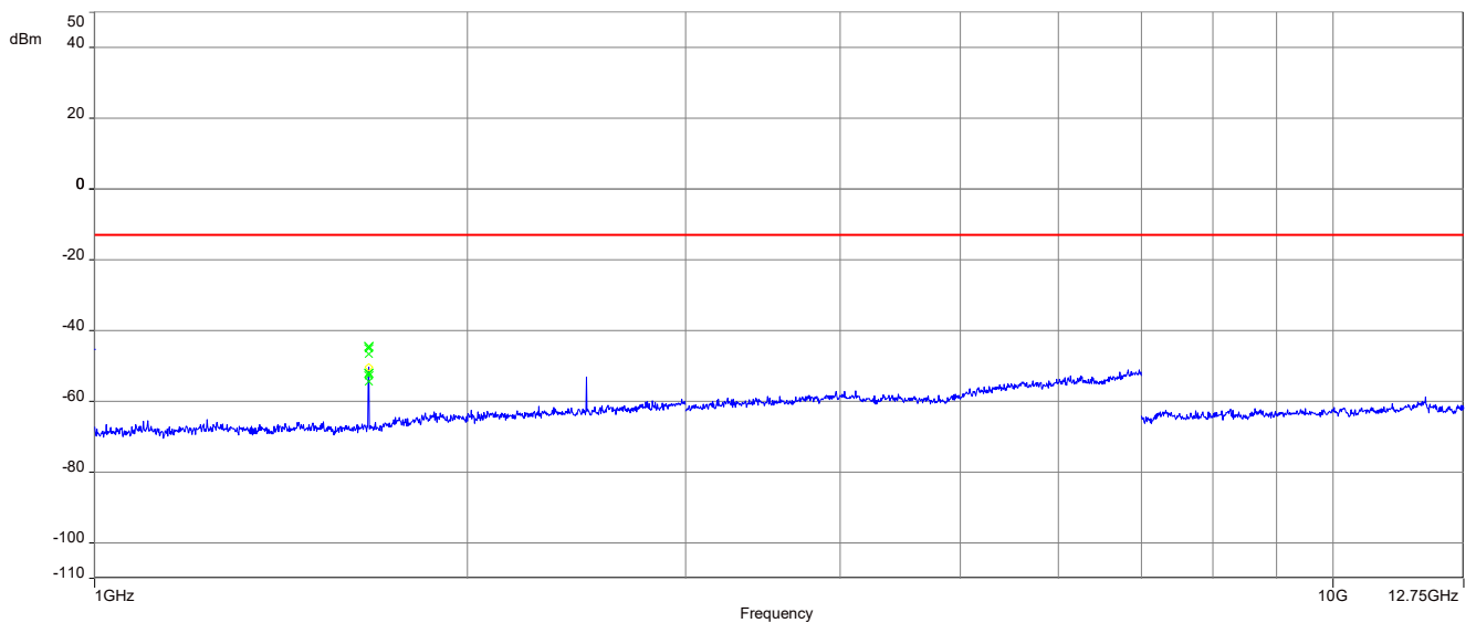
Plot 6: Middle channel (1 GHz – 12.75 GHz), LTE band 5
