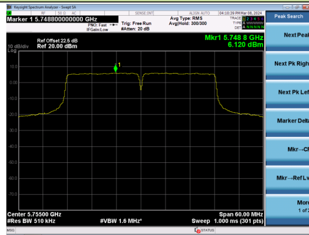
Channel 151 (5755MHz)
