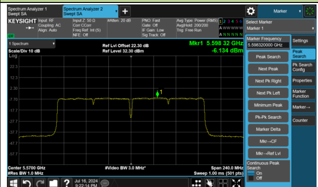
Channel 114 (5570MHz)
