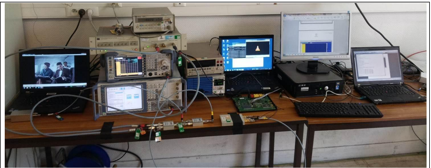
Photograph for DFS U-NII Detection Bandwidth
