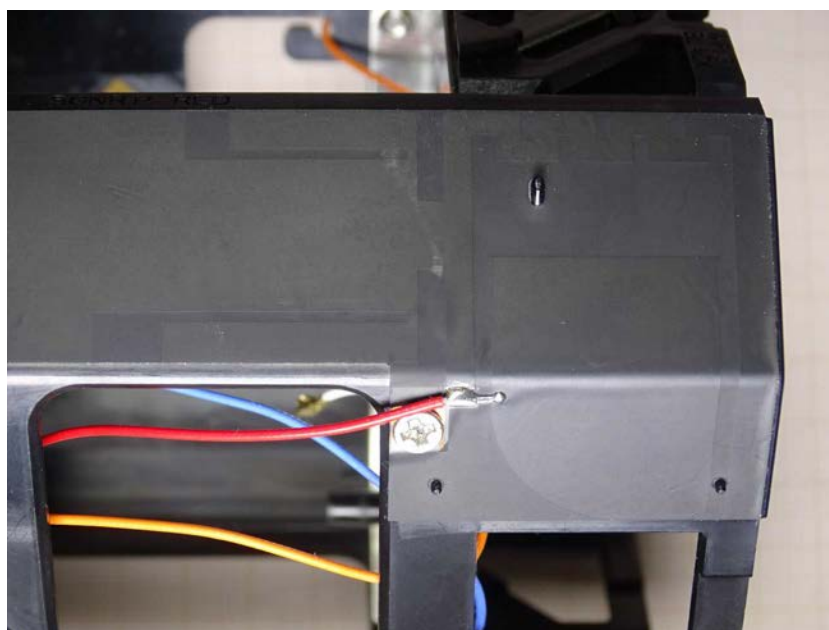
Photo 34 - 4G/5G antenna
