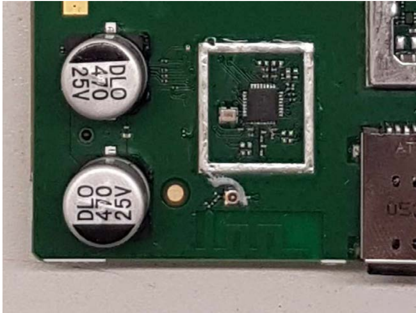
Photo 27 - BT antenna
