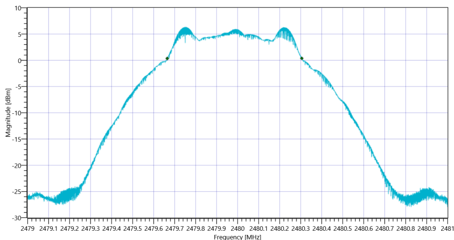
FCC Part 15.247 Maximum Peak Conducted Output Power DTS ~ BT LE 1 Msp DTS BW
