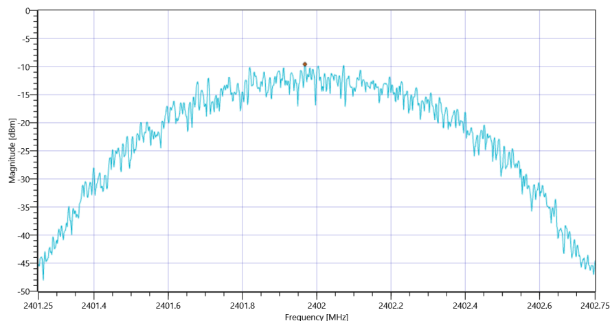
FCC Part 15.247 Peak Power Spectral Density DTS ~ BT LE 1 Mbps
