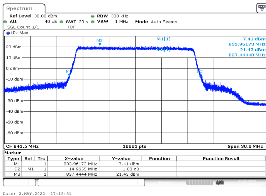
Plot 60: 15 MHz – 16-QAM - highest channel (-26 dBc BW)
