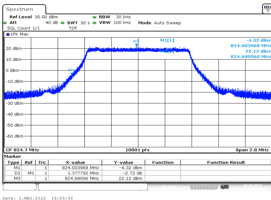
Plot 32: 1.4 MHz – 16-QAM - lowest channel (-26 dBc BW)
