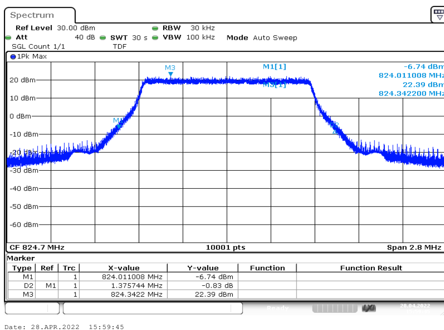
Plot 62: 1.4 MHz – 64-QAM - lowest channel (-26 dBc BW)
