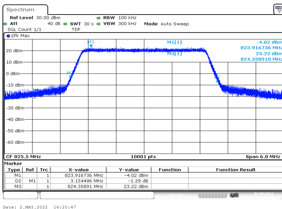
Plot 38: 3 MHz – 16-QAM - lowest channel (-26 dBc BW)
