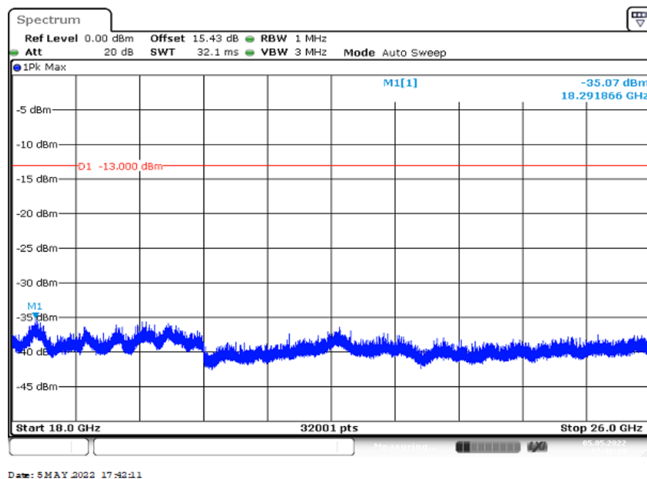
Plot 8: 16-QAM - Middle channel (18 GHz – 26 GHz)
