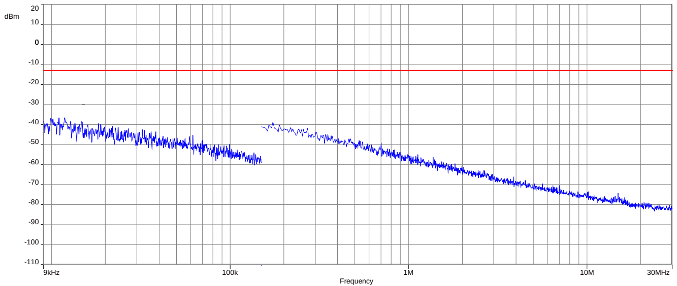
Plot 13: BPSK - Middle channel (9 kHz - 30 MHz)
