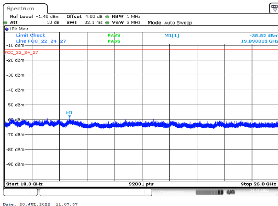
Plot 20: 256-QAM - Middle channel (18 GHz – 26 GHz)
