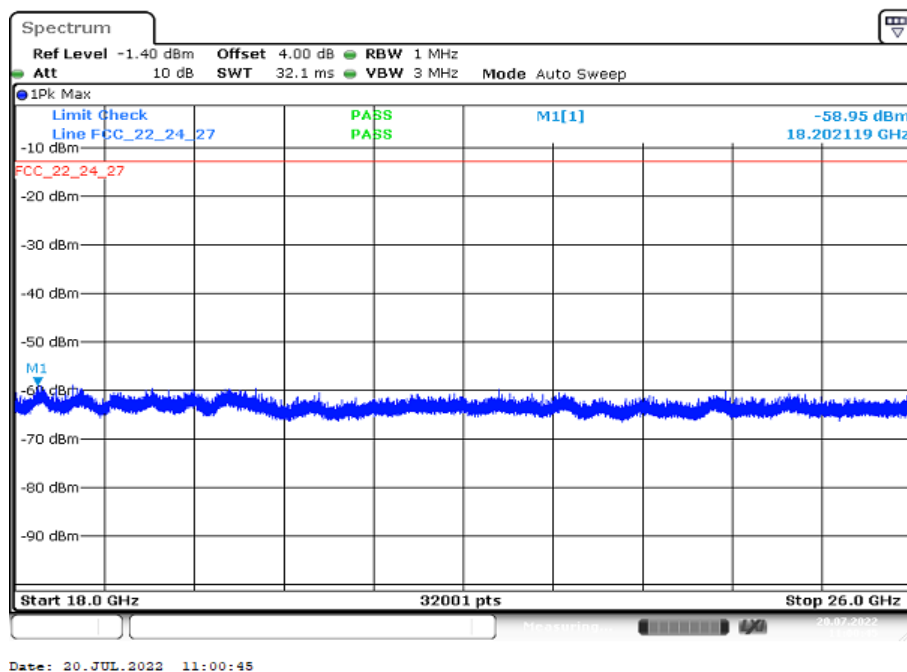
Plot 16: BPSK - Middle channel (18 GHz – 26 GHz)
