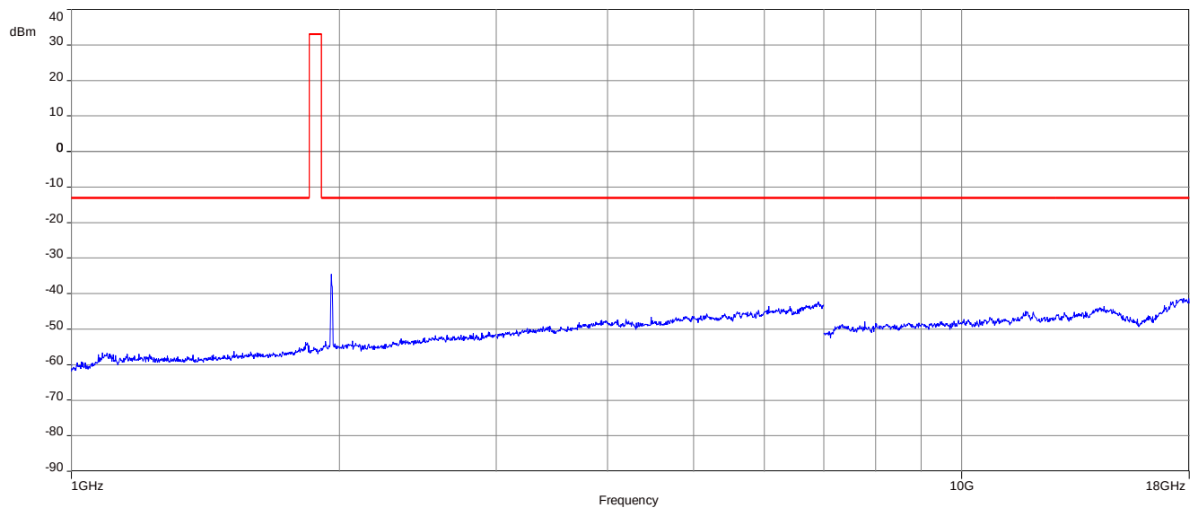
Plot 11: 64-QAM - Middle channel (1 GHz – 18 GHz)
