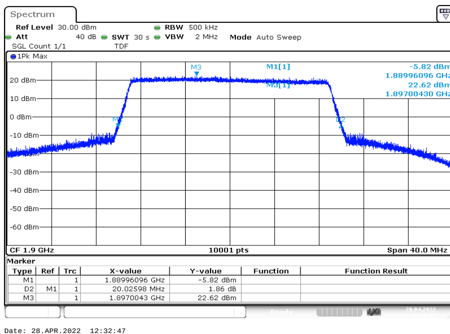
Plot 108: 20 MHz – 64-QAM - highest channel (-26 dBc BW)
