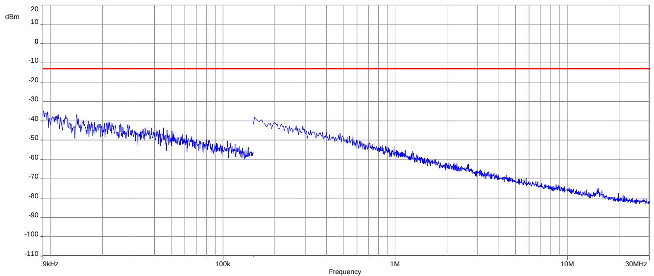
Plot 10: BPSK - Middle channel (9 kHz - 30 MHz)
