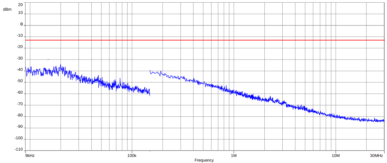
Plot 7: 64-QAM - Middle channel (9 kHz - 30 MHz)
