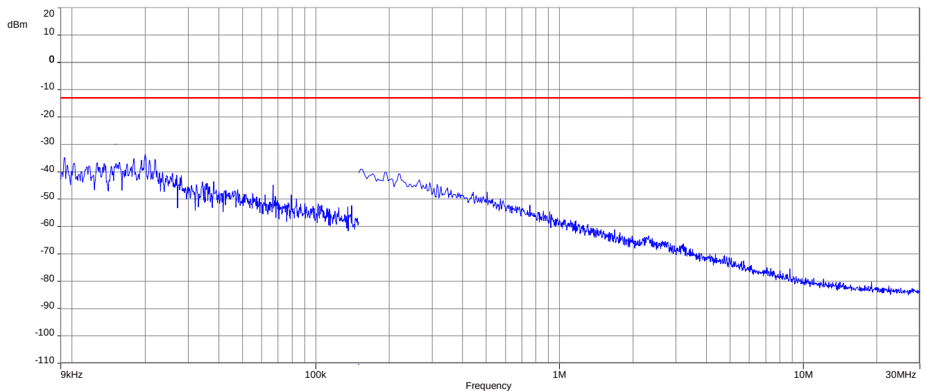
Plot 4: 16-QAM - Middle channel (9 kHz - 30 MHz)
