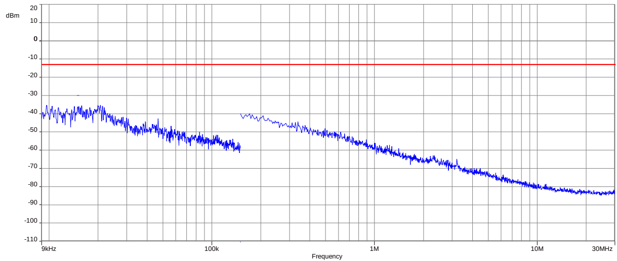
Plot 1: QPSK - Middle channel (9 kHz - 30 MHz)
