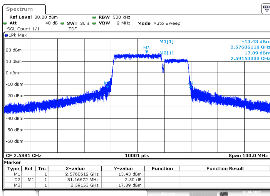
Plot 8: 20 MHz + 10 MHz– QPSK - middle channel (-26 dBc BW)
