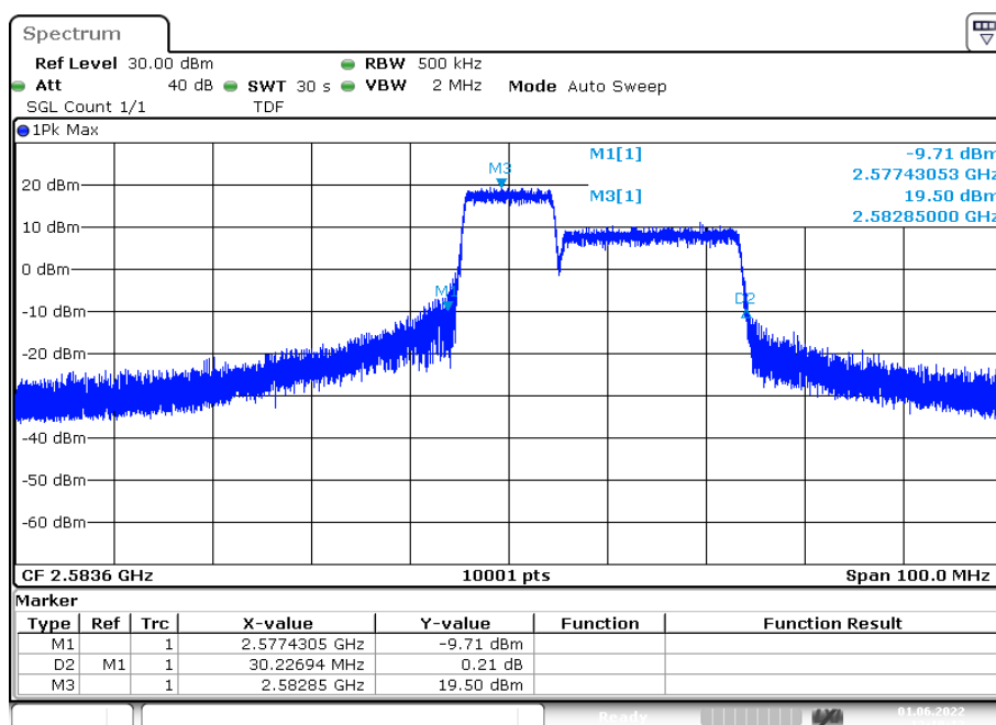
Plot 6: 10 MHz + 20 MHz– QPSK - middle channel (-26 dBc BW)
