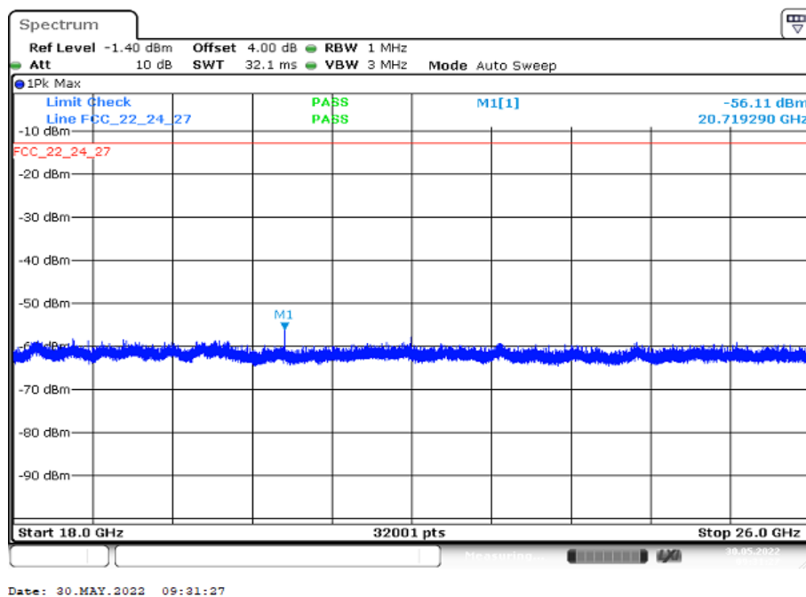
Plot 16: 256-QAM - Middle channel (18 GHz – 26 GHz)
