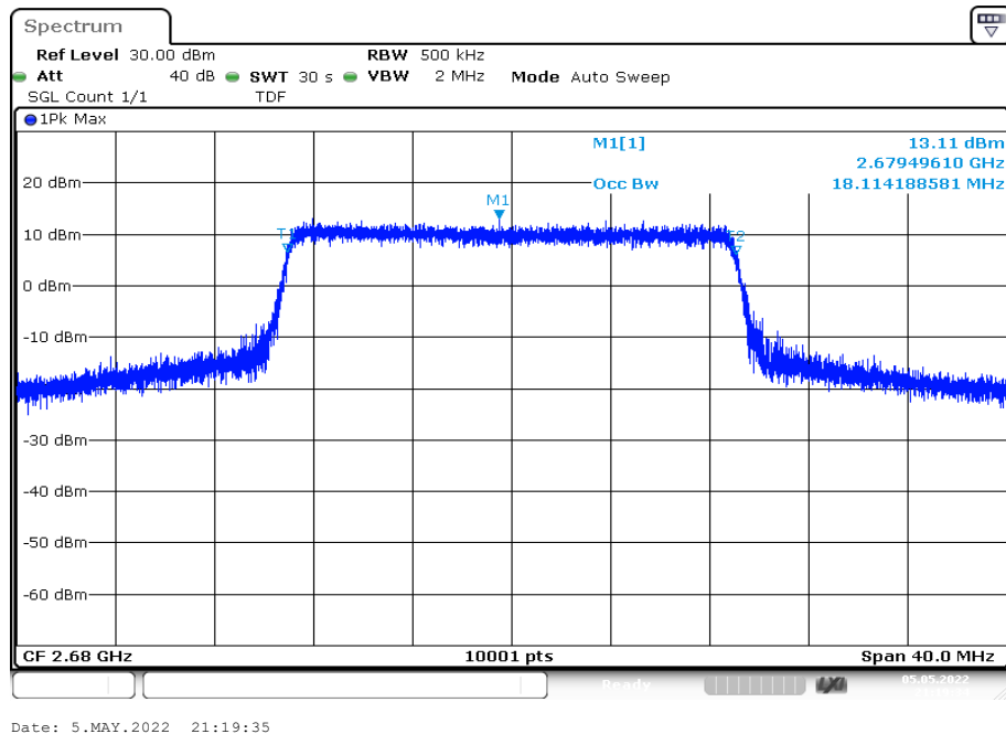
Plot 47: 20 MHz – 16-QAM - highest channel (99% - OBW)
