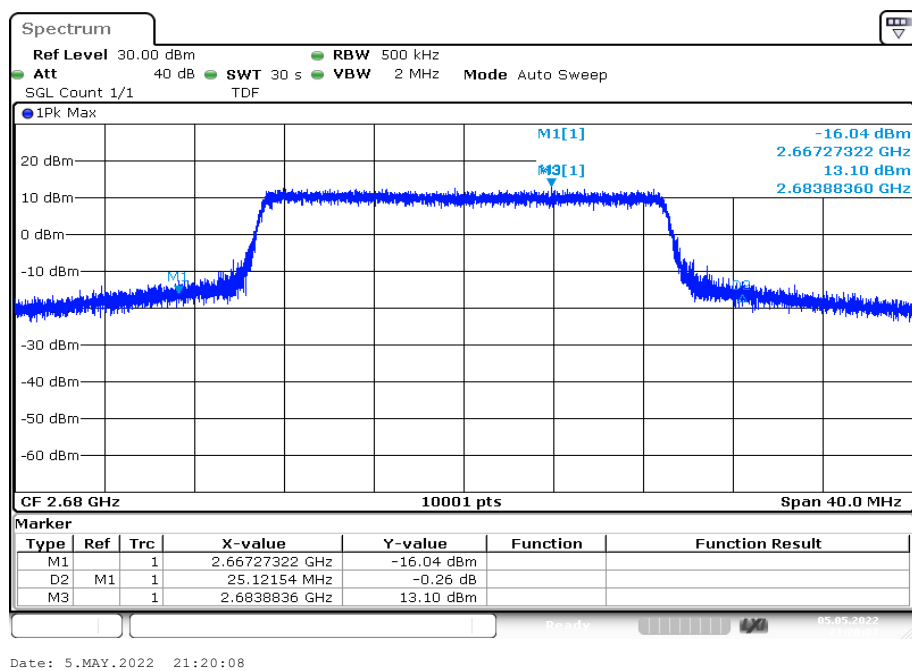
Plot 48: 20 MHz – 16-QAM - highest channel (-26 dBc BW)
