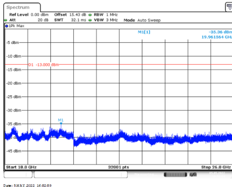
Plot 4: QPSK - Middle channel (18 GHz – 26 GHz)
