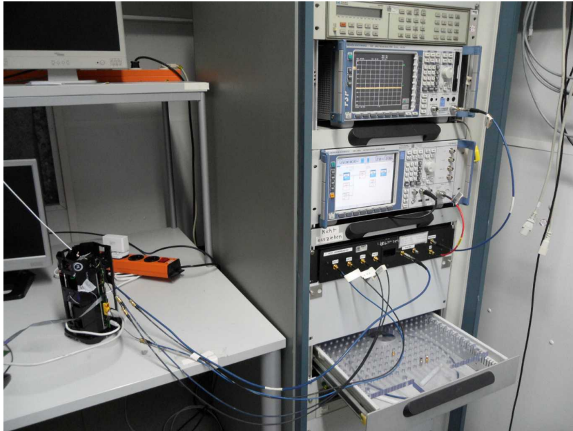
Photo 9: DFS test setup
