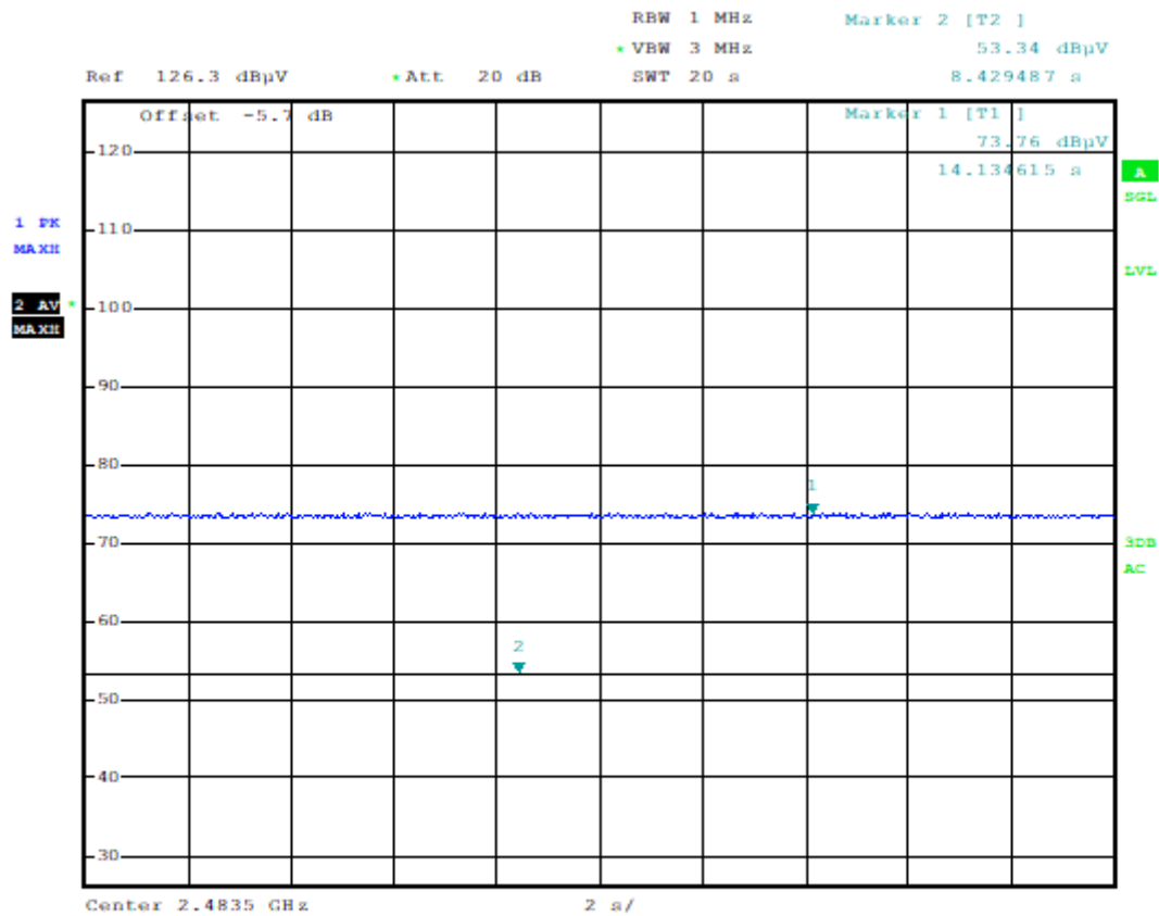
Plot 3: Upper restricted band, 1 Msps, detailed plot
