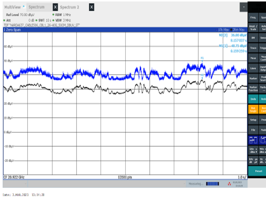
Plot 13: Worst case Peak to Average (Zero Span)
