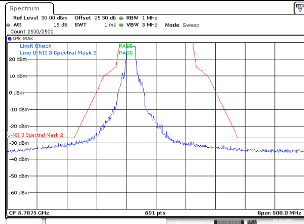
Antenna 1
