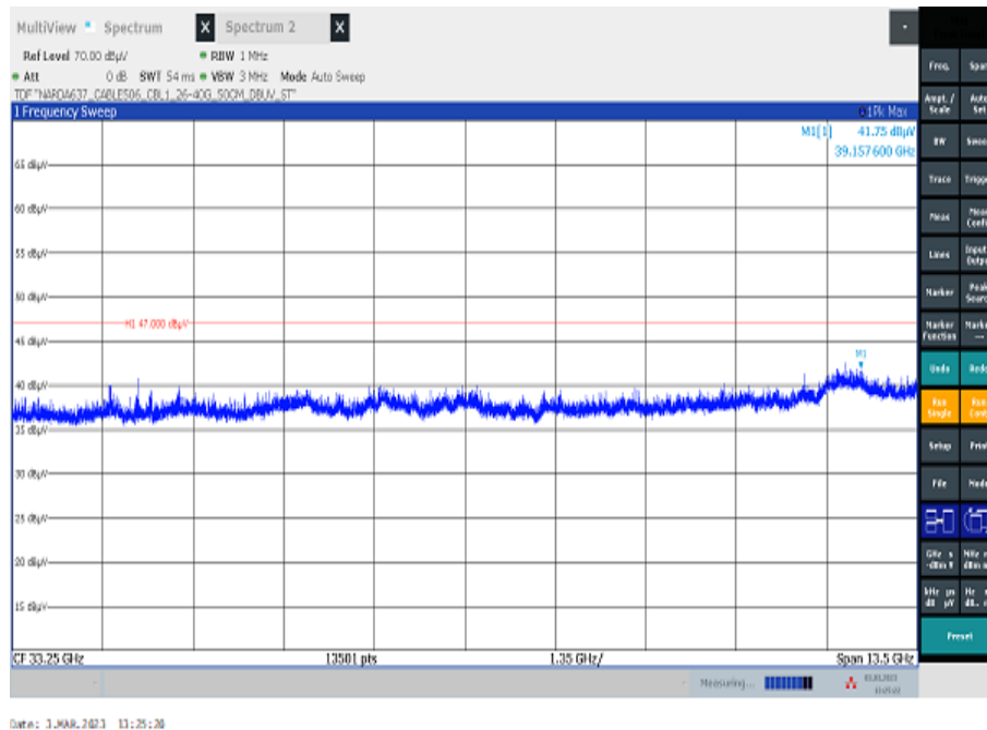
Plot 15: 26 GHz to 40 GHz, vertical & horizontal polarization, valid for all channels
