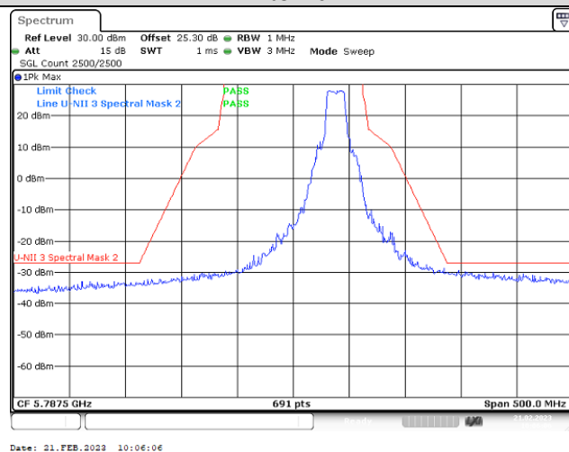
Antenna 1
