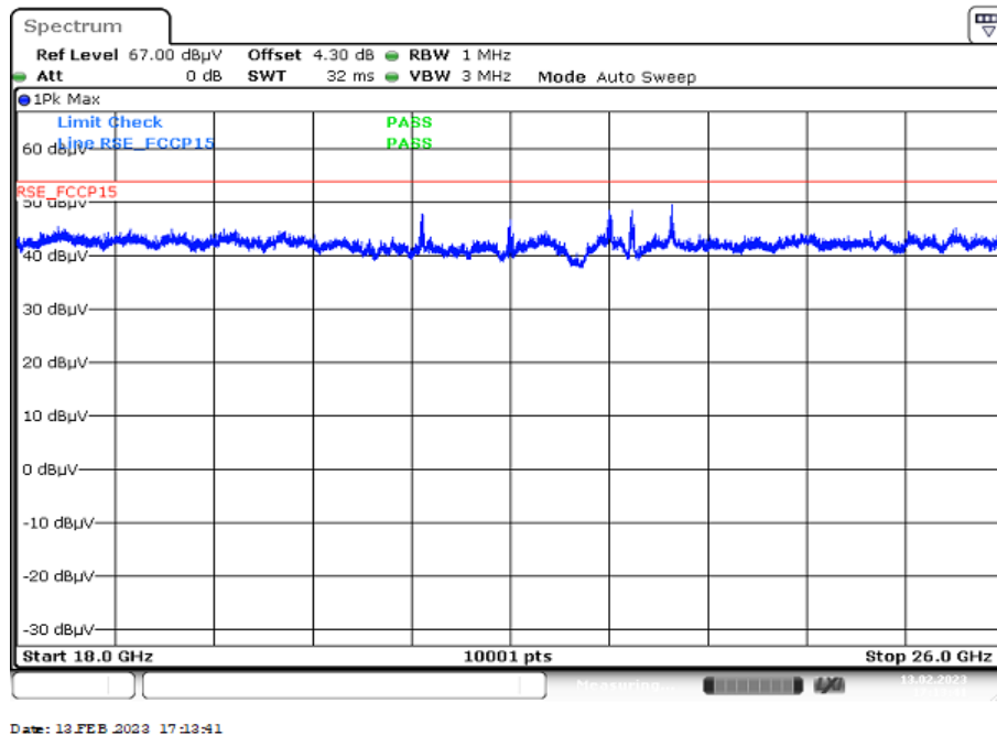
Plot 11: 18 GHz to 26 GHz, vertical & horizontal polarization, valid for all channels
