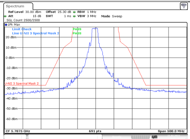
Antenna 1
