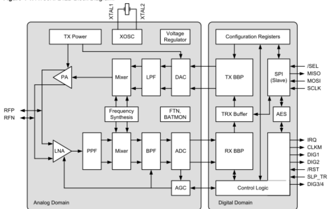
Figure 4-1. AT86RF212B Block Diagram.
