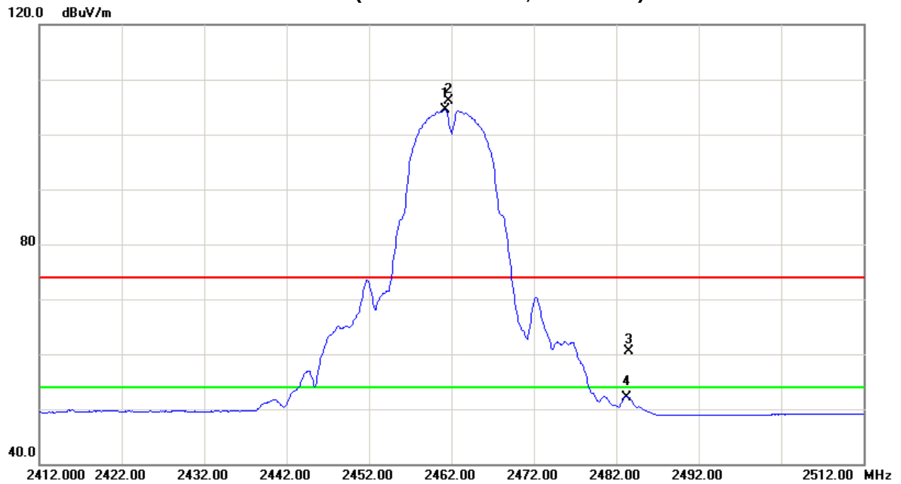
TX CH11 (Above 1000 MHz, Horizontal)
