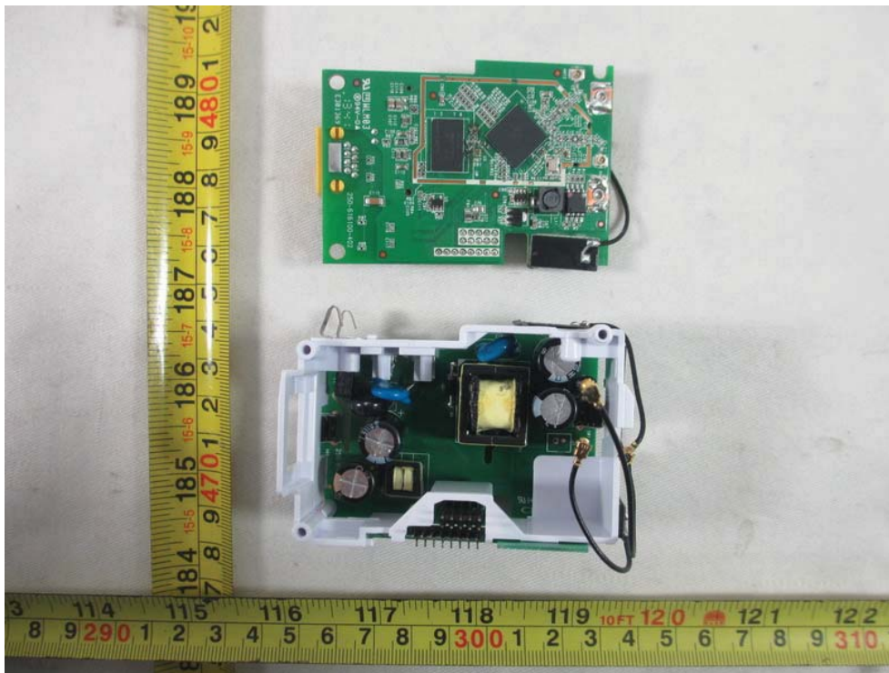
main board
