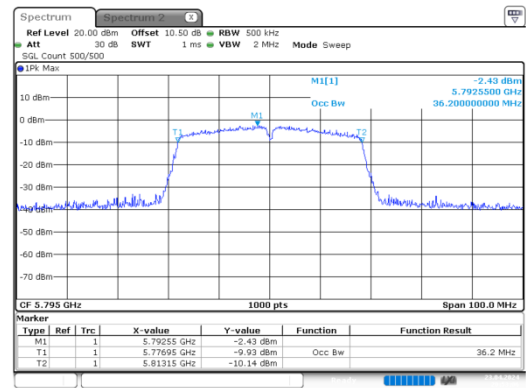
n40_5795MHz_Chain 0
