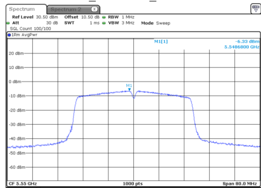
n40_5550MHz_Chain 0
