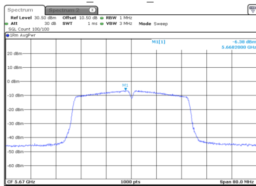
n40_5670MHz_Chain 0
