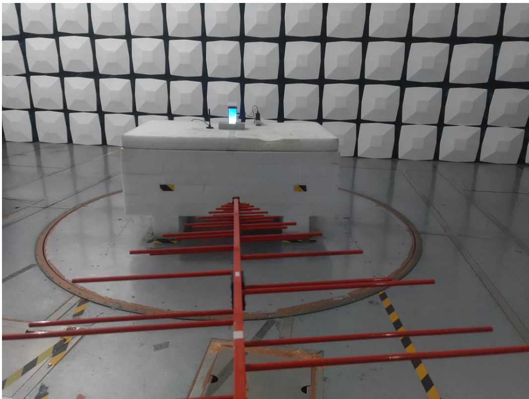
Radiated Emission 30M-1GHz View Test Mode:S1 Plus
