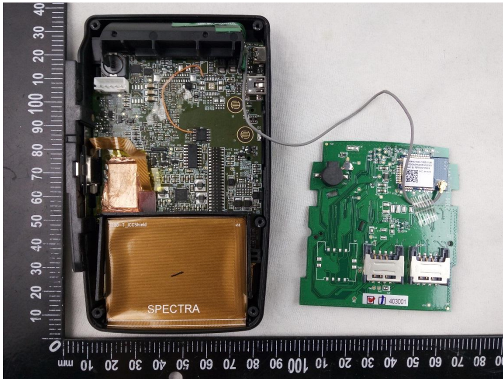
EUT MODEL T300 UNCOVER VIEW 3
