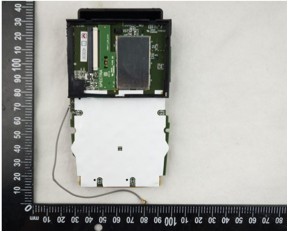
EUT MODEL T300 UNCOVER VIEW 5
