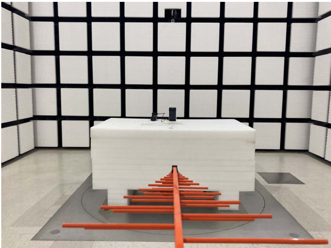
Radiated Emission Below 1G View
