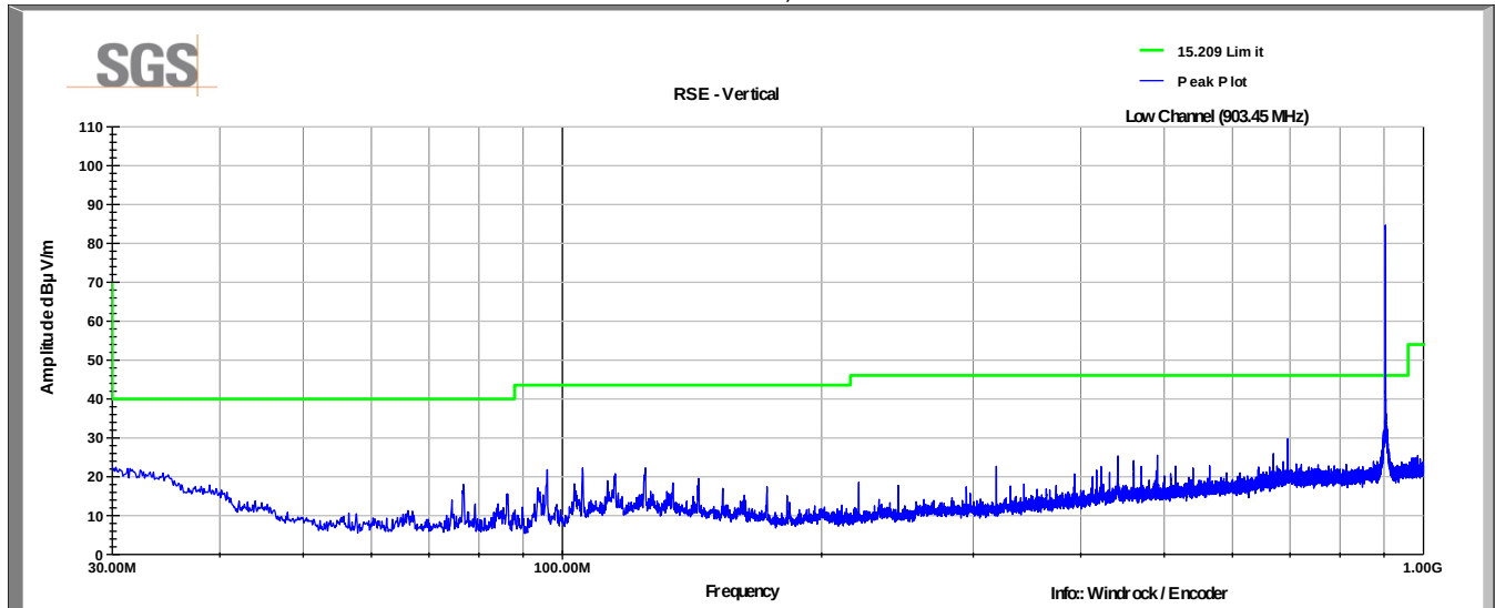
Low Channel, 903.45 MHz 30-1000MHz, Vertical
