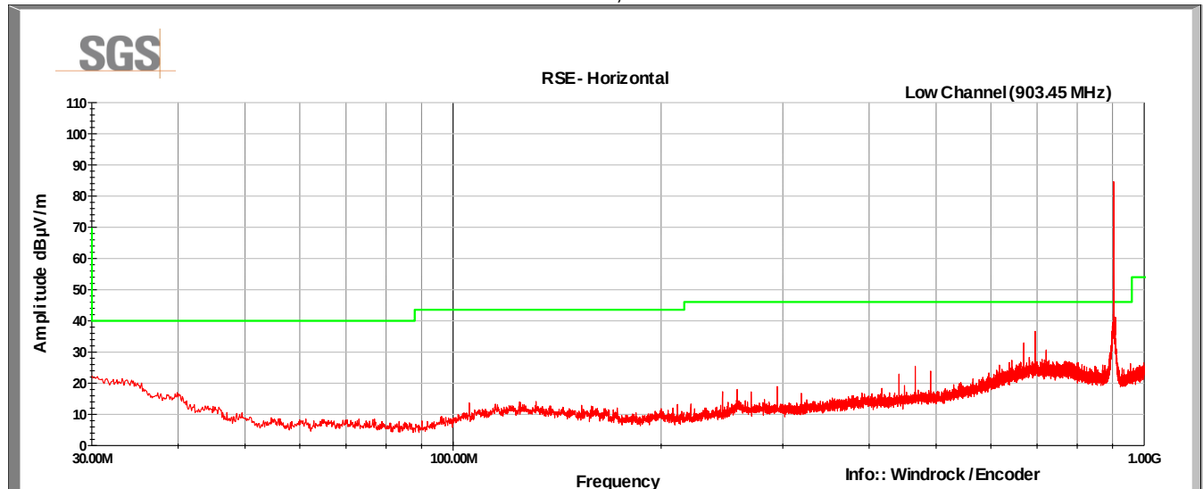
Low Channel, 903.45 MHz 30-1000MHz, Horizontal
