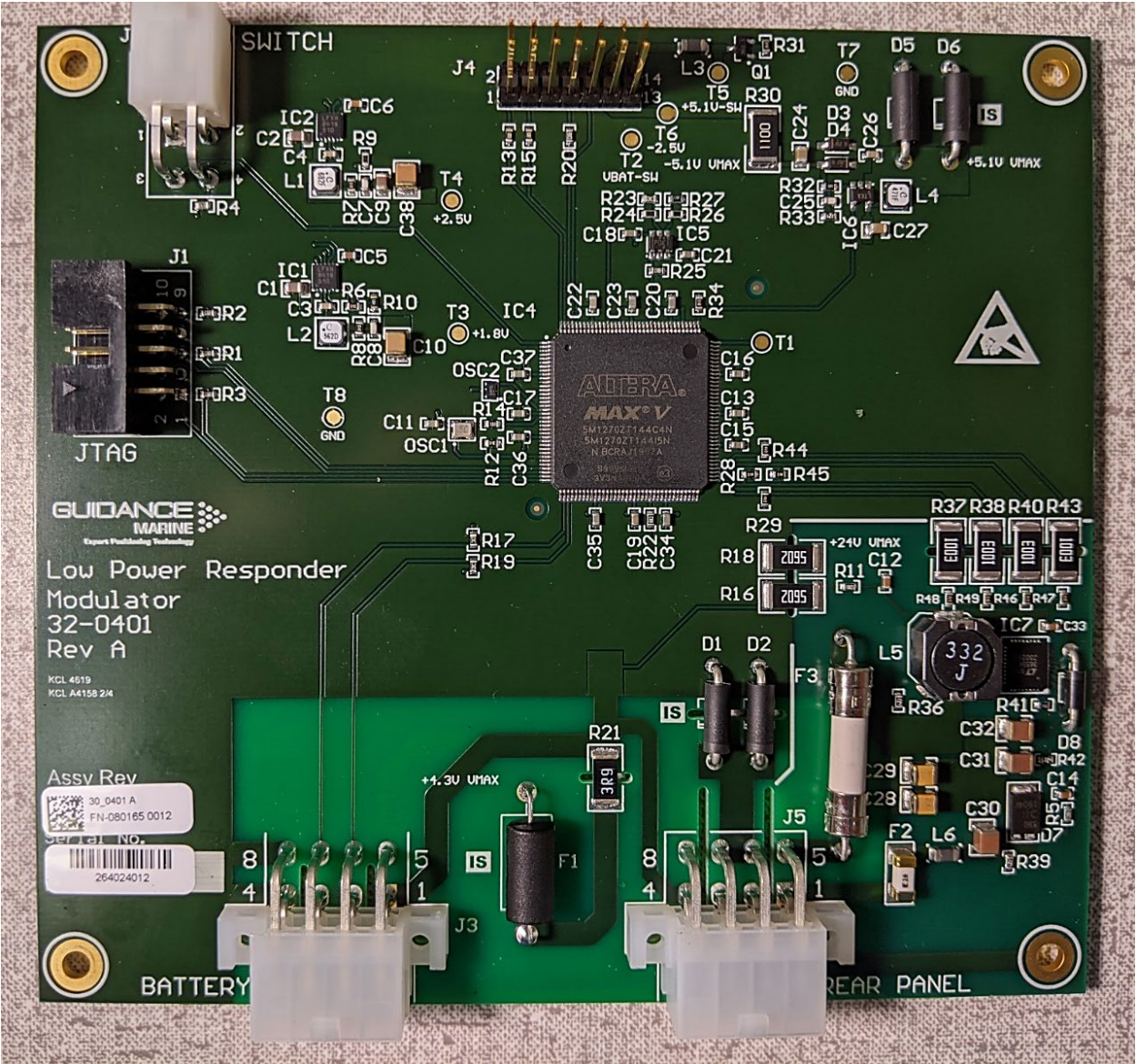
Control PCB, Front
