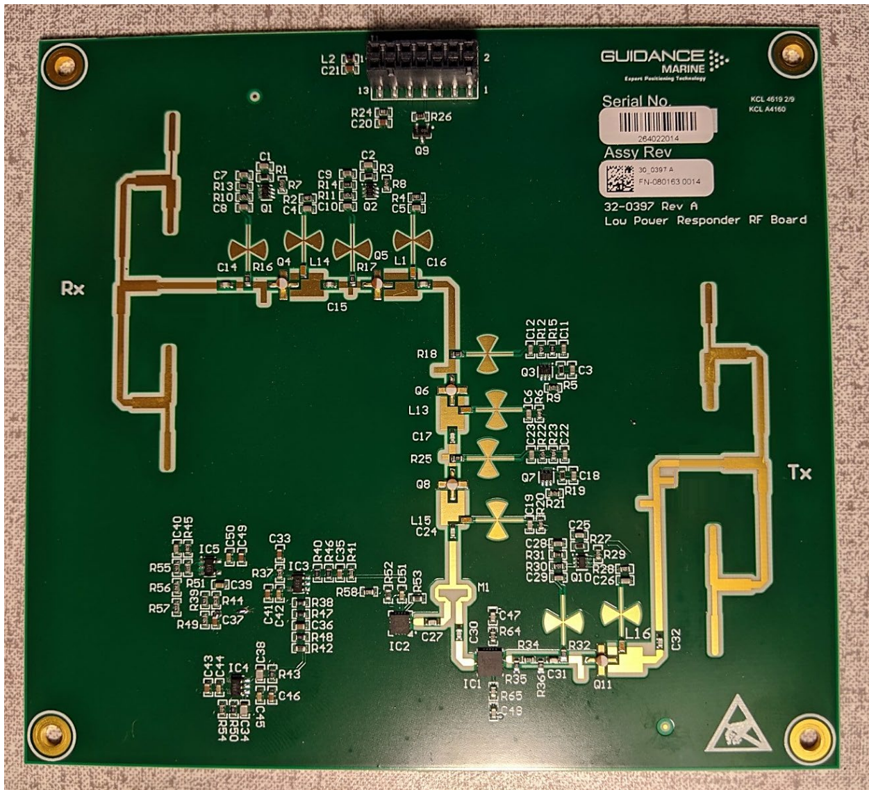
Antenna PCB, Back
