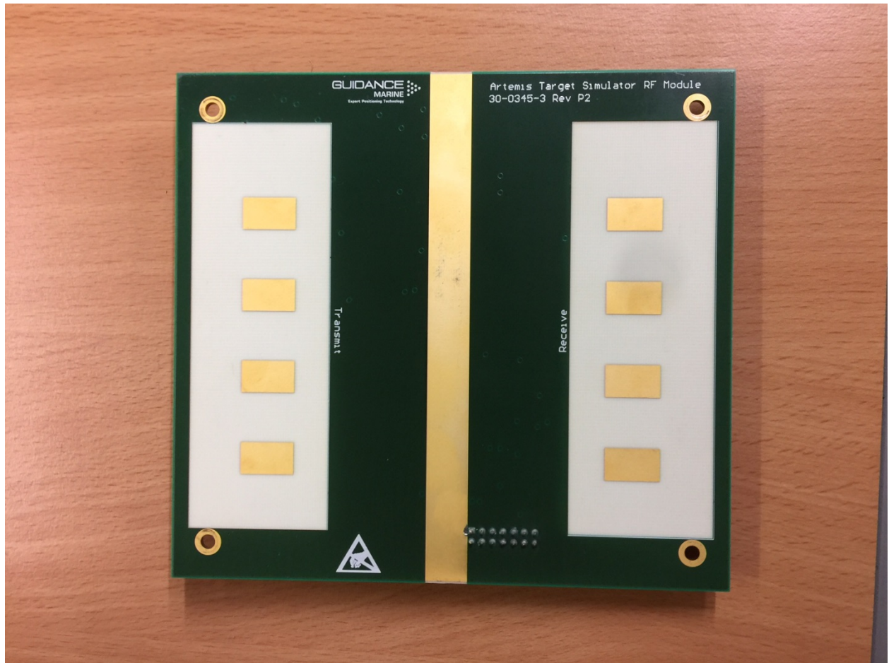
FRONT VIEW RF BOARD
