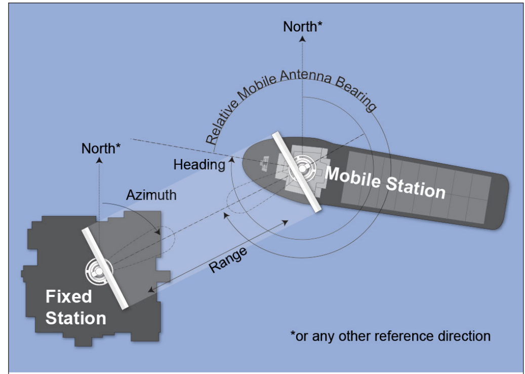
Layout of a Standard Artemis System
