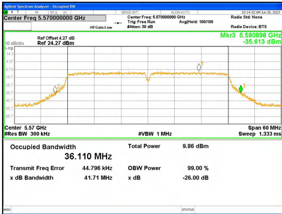
-26dB Bandwidth NVNT ac40 5570MHz Ant2
