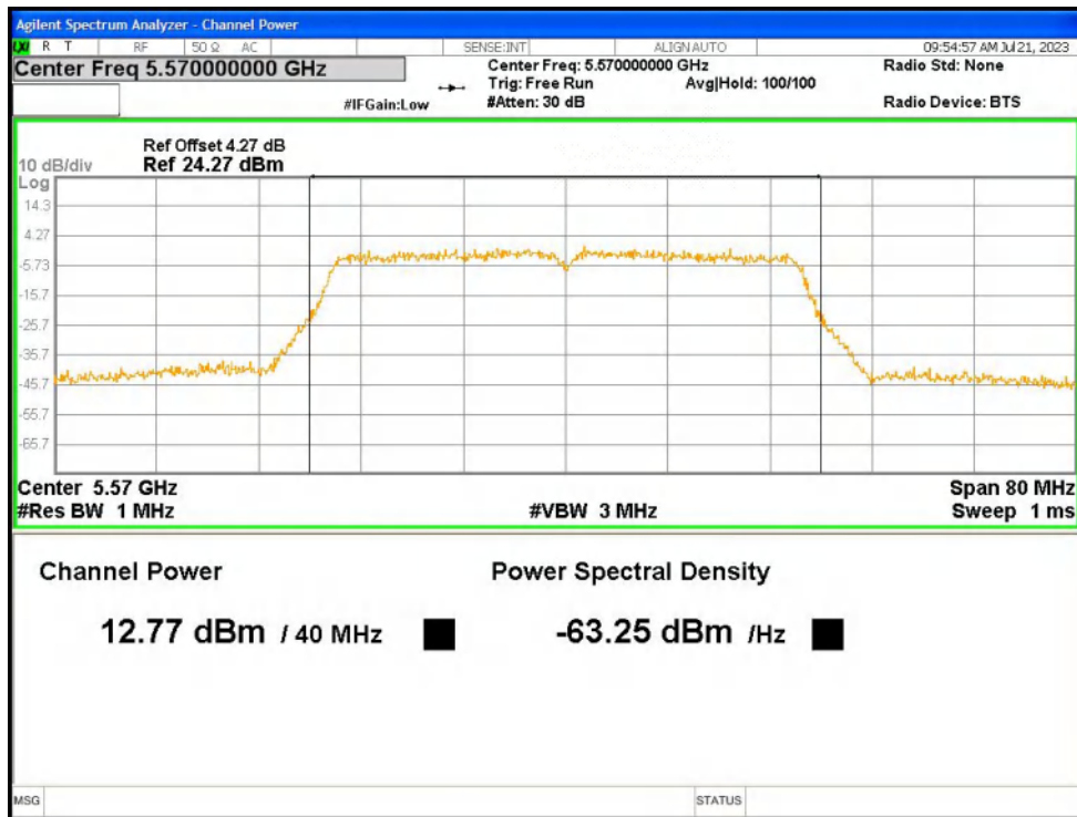
Power NVNT n40 5570MHz Ant2
