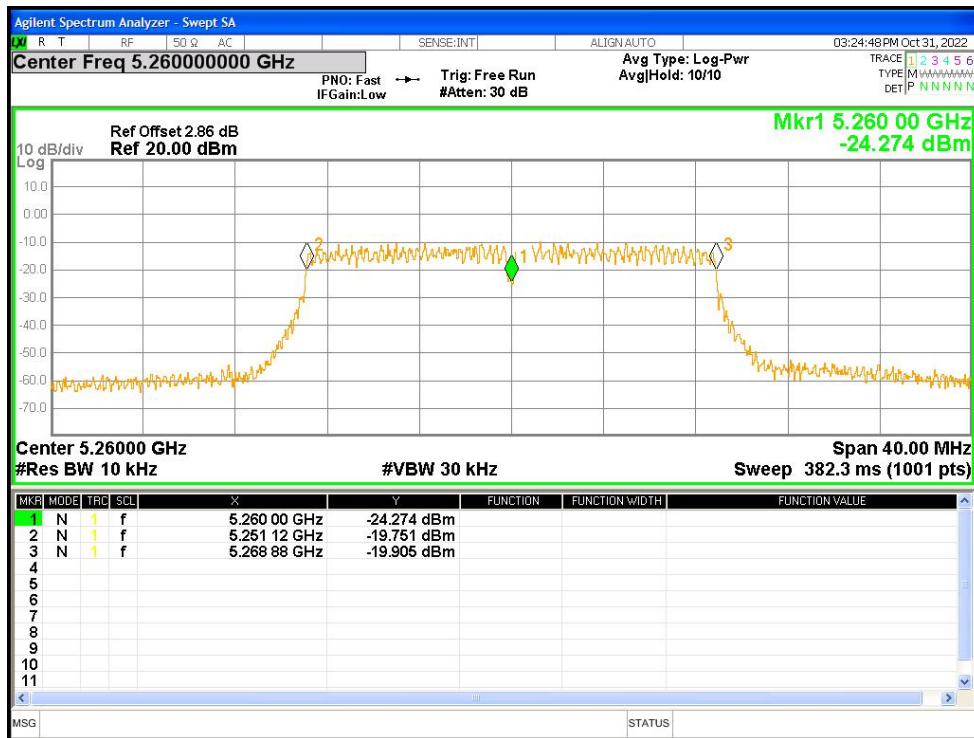
Freq. Stability NVNT ac20 5280MHz Ant2
