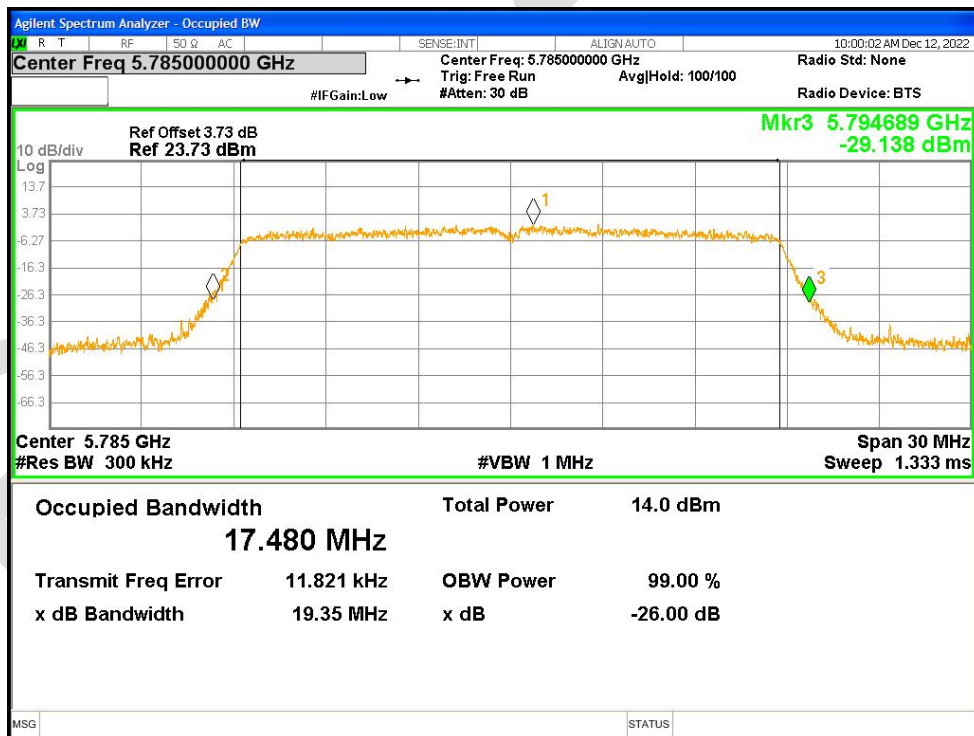
-26dB Bandwidth NVNT n20 5785MHz Ant2
