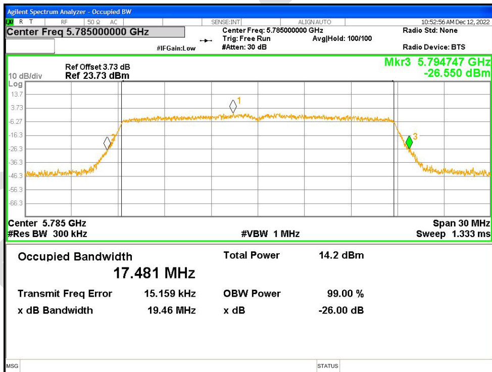
-26dB Bandwidth NVNT ac20 5785MHz Ant2
