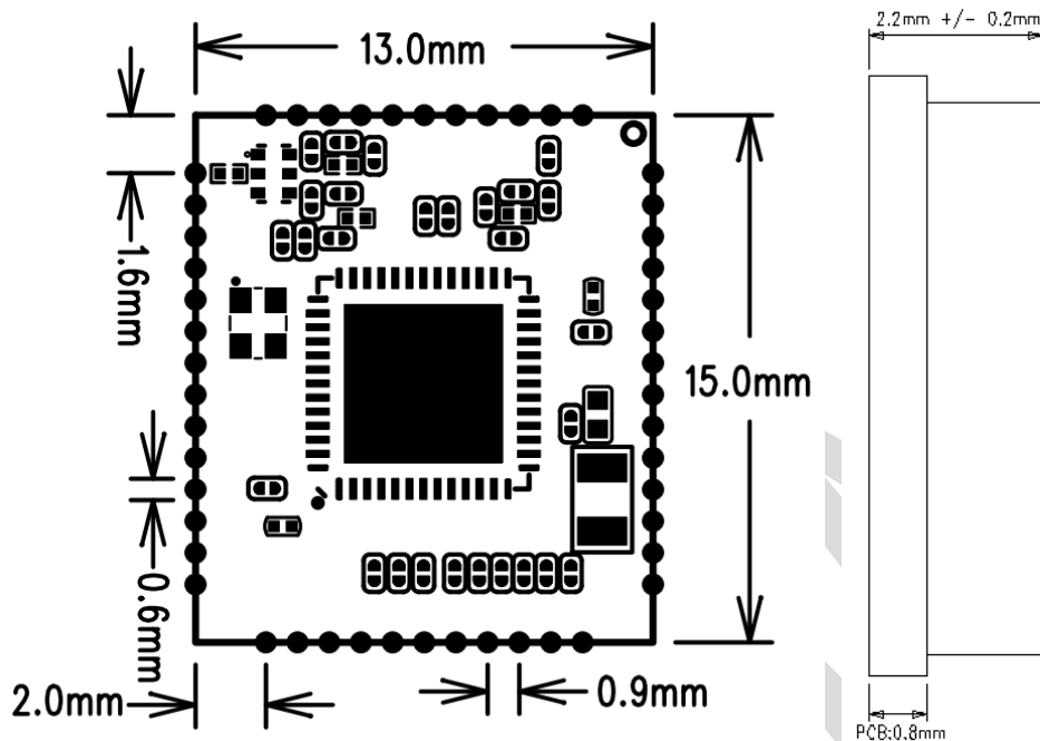
Figure 4. Mechanical Size of AW3155-50
