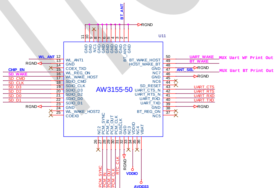
Figure 3. Application Circuit Diagram of AW3155-50
