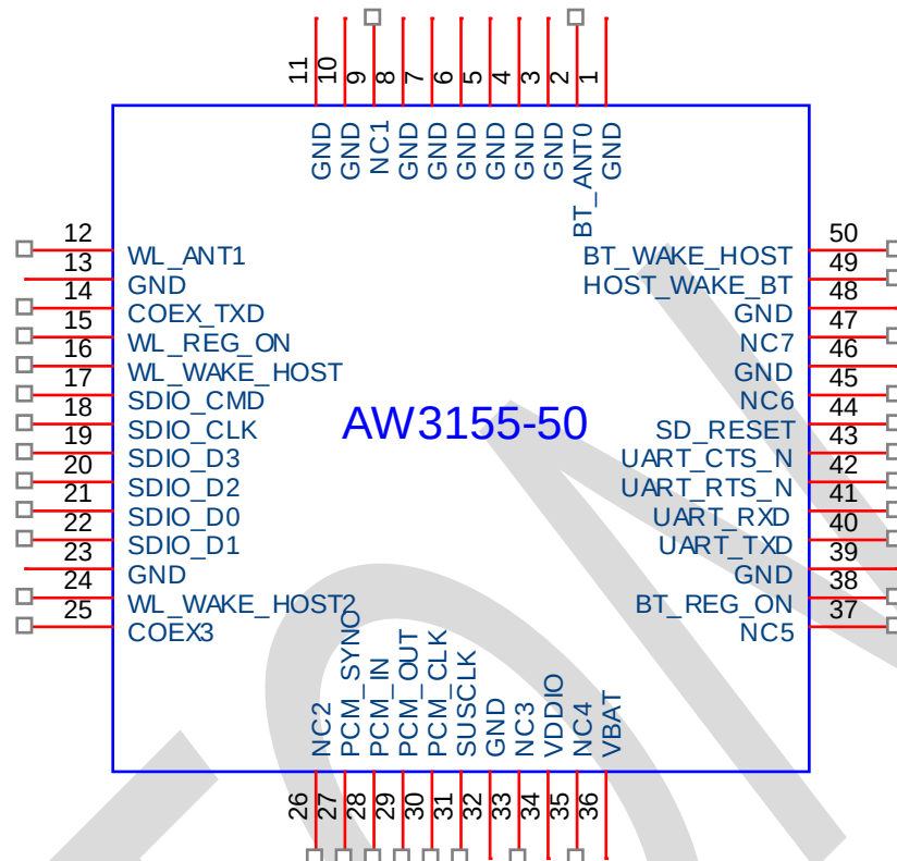
Figure 2.Pin Diagram of AW3155-50
