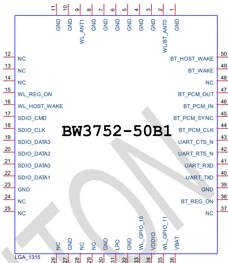
Figure 2.Pin Diagram of BW3752-50B1
