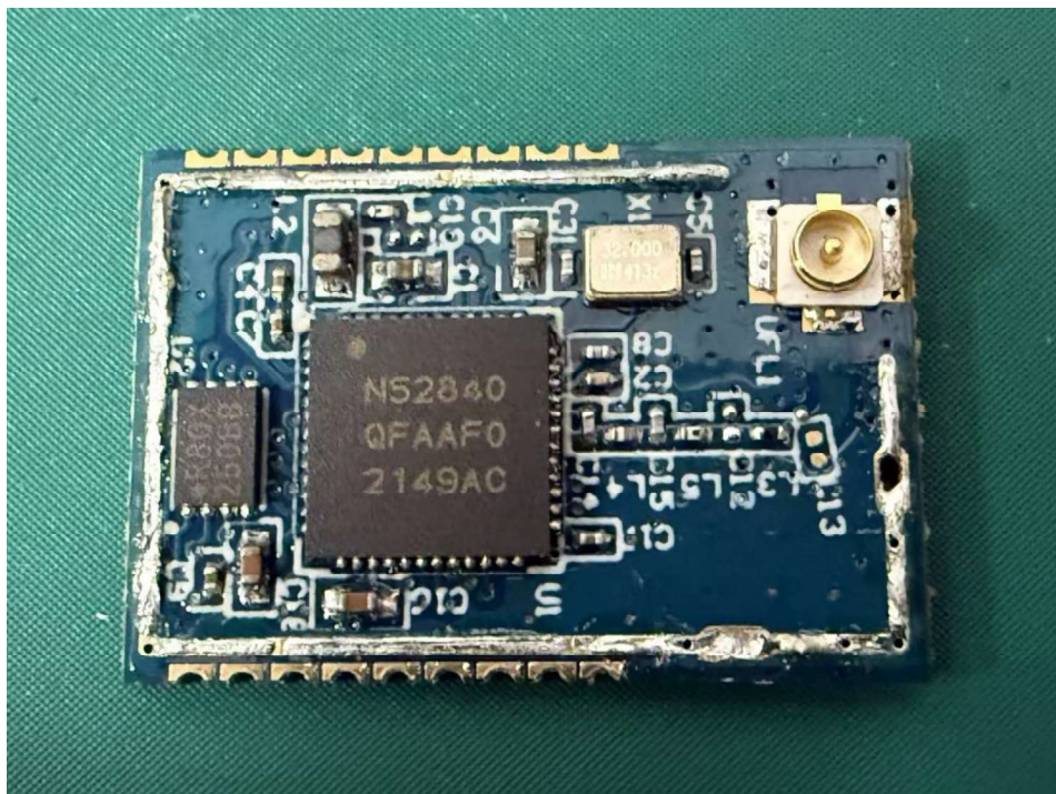
Internal: PCB
