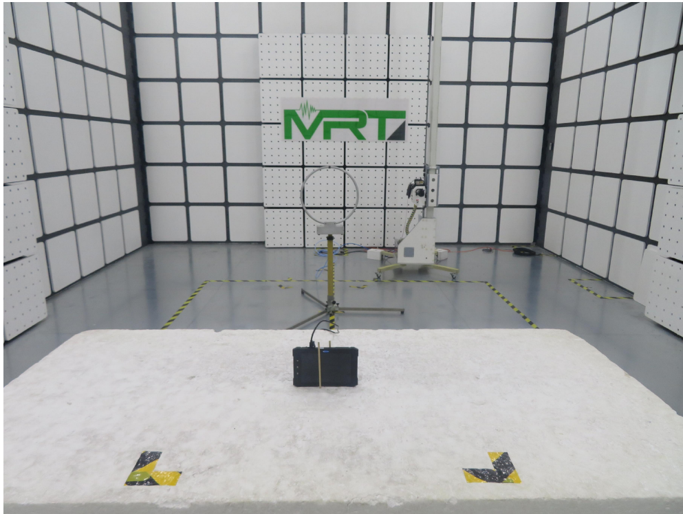
Description: Radiated Emission Test Setup for 150kHz ~ 30MHz
