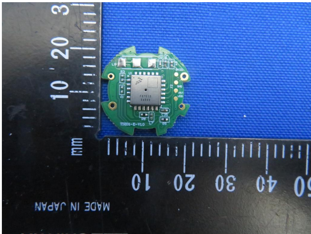
(16) EUT Photo (3685A)
