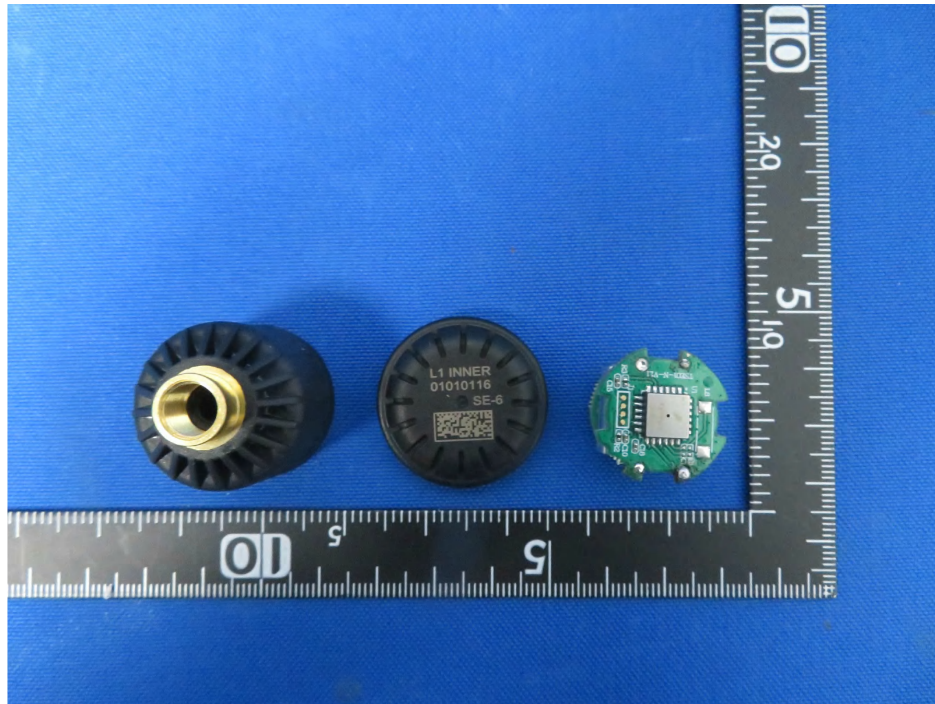
(1) EUT Photo
