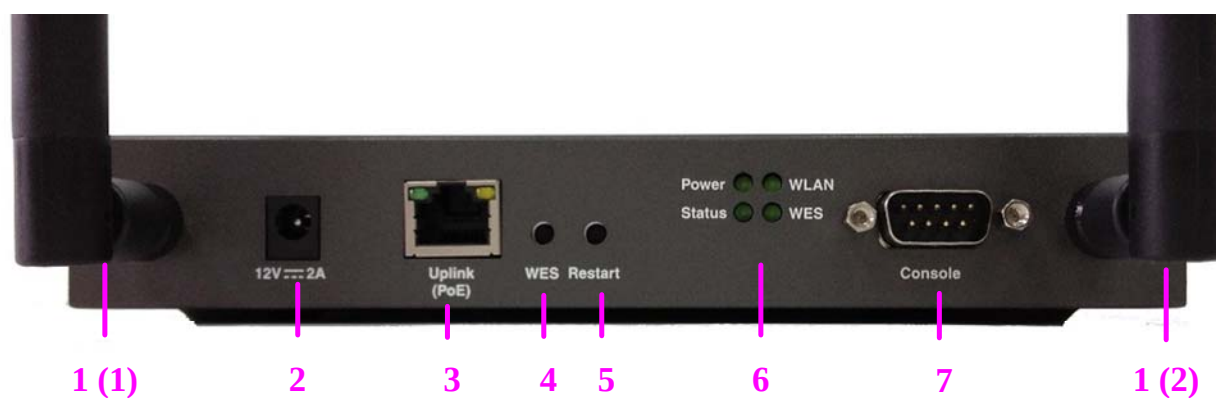
Figure 2 EAP210 Rear Panel
