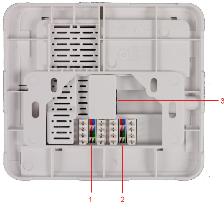
EAP705 back Panel
