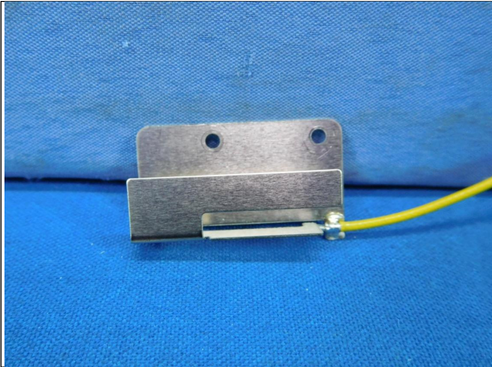
Antenna 3
