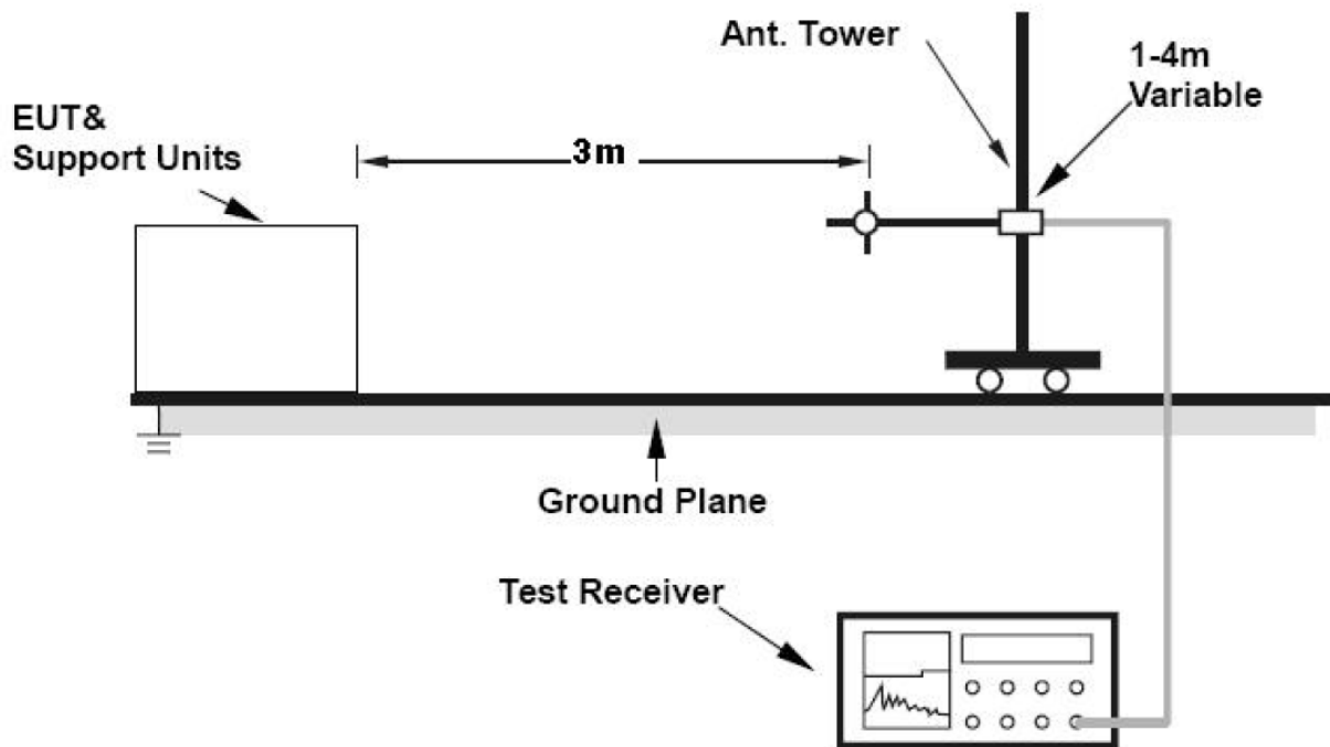
Figure – 2 Test setup for Radiated emissions
