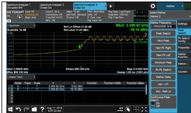
Band Edge-Hopping-2401.5MHz
