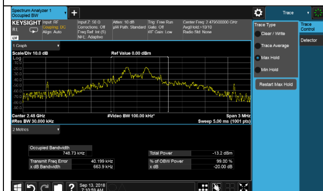
99% and 20dB BW – 2479.5MHz
