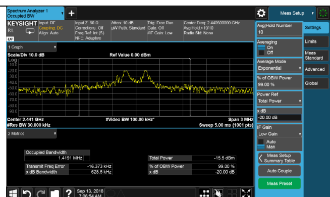
99% and 20dB BW – 2440.5MHz
