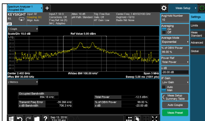
99% and 20dB BW – 2401.5MHz
