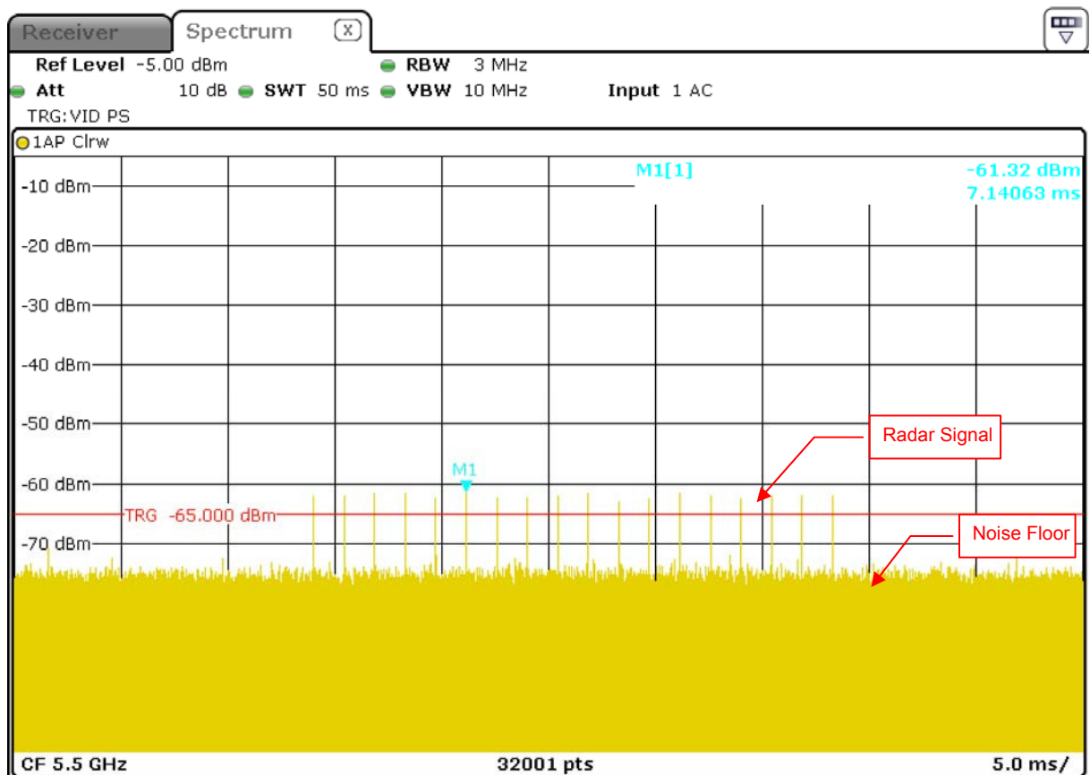
Radar Signal 0
