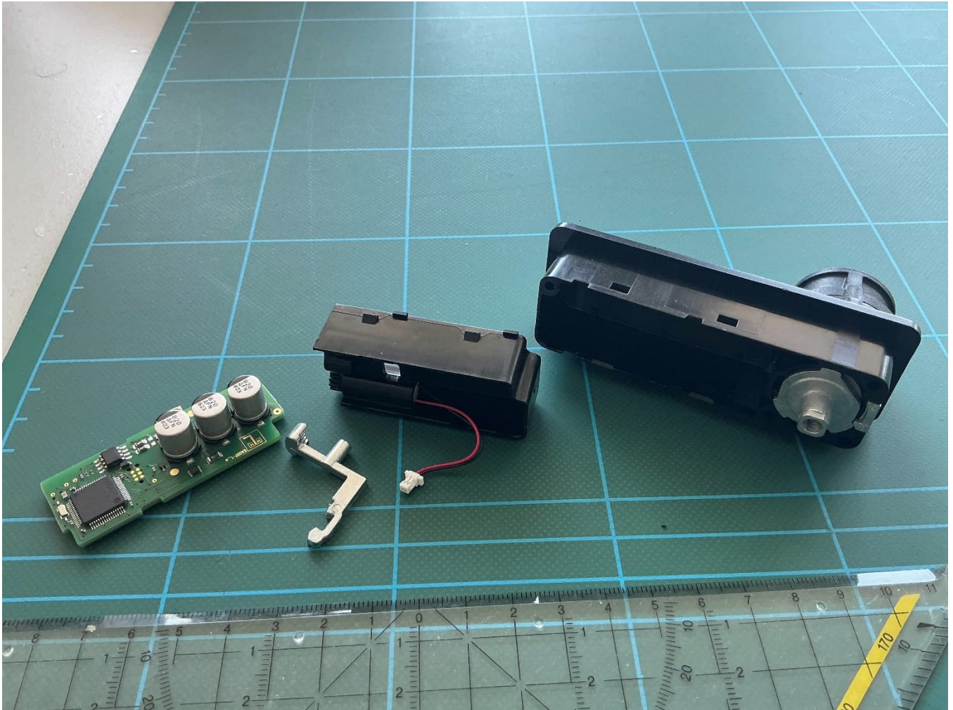
EUT, housing opened and PCB removed
