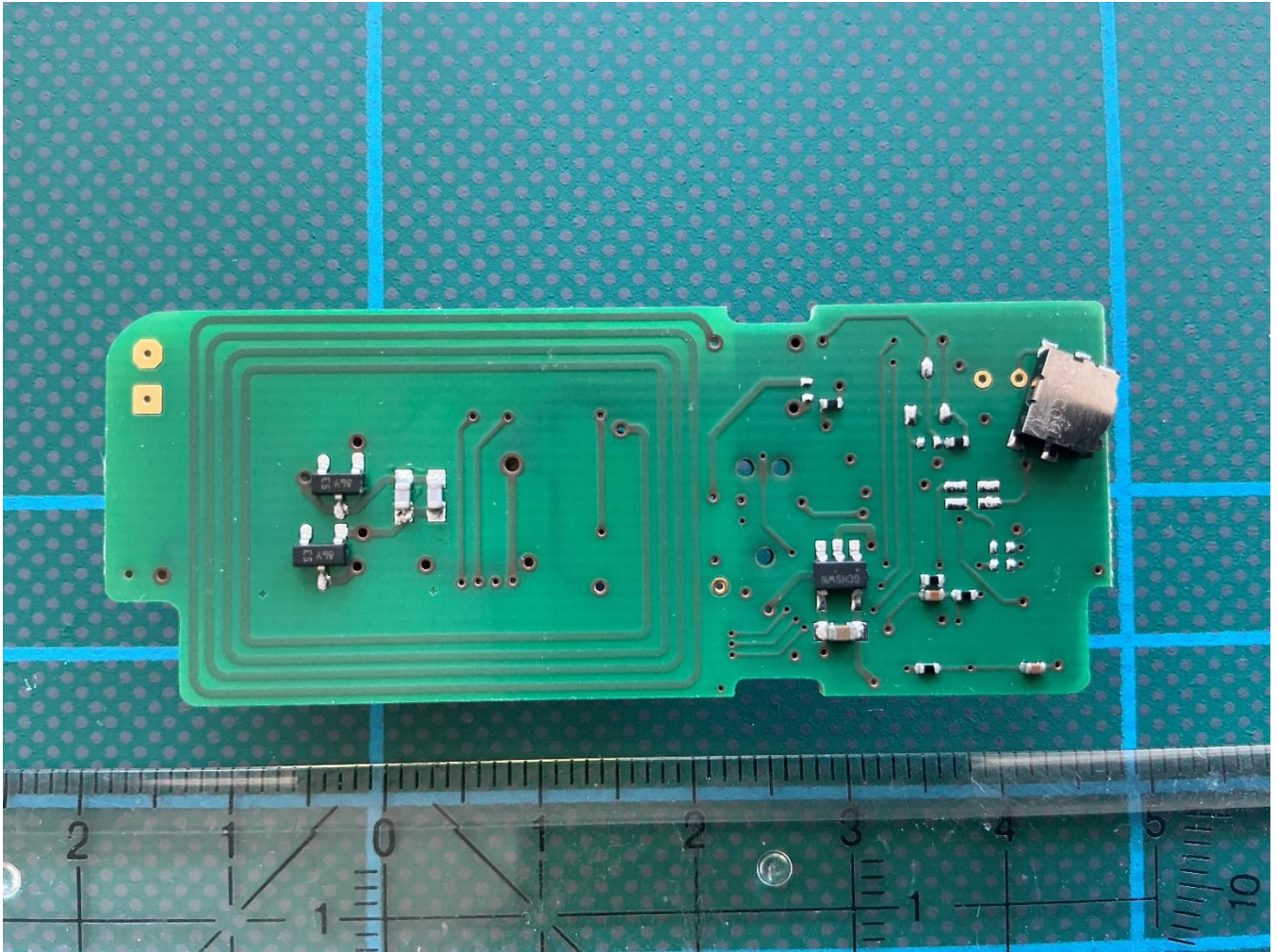
PCB, bottom view
