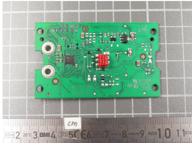
TA03, PCB, front view
