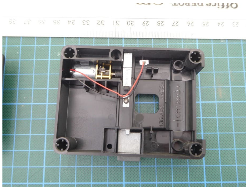
M420 PRO, housing opened, view 3
