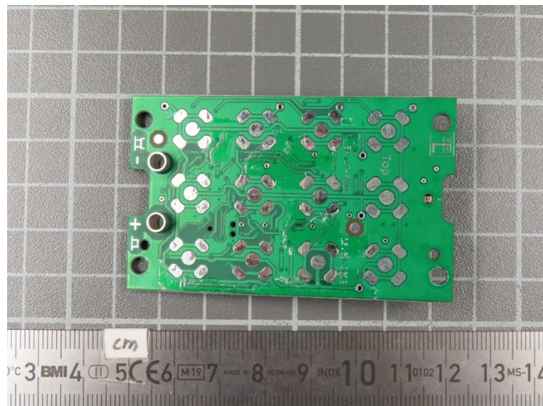
TA03, PCB, back view
