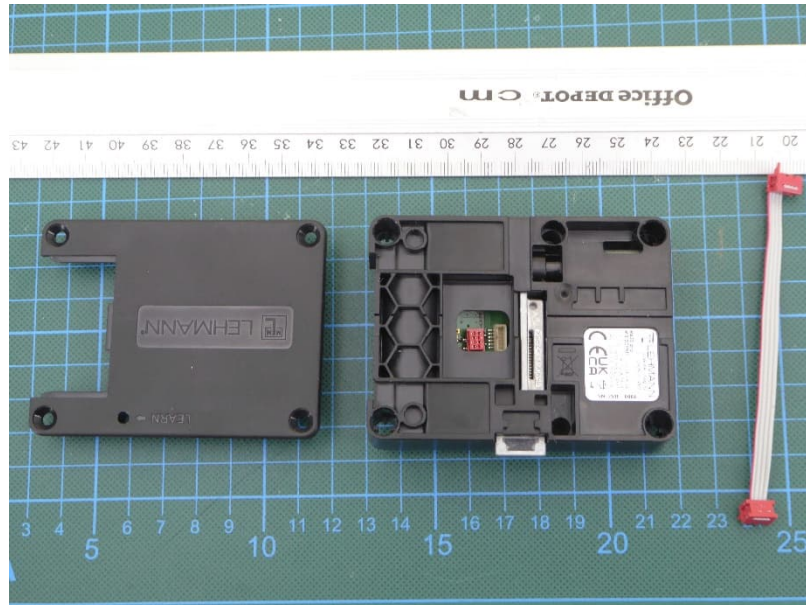
M420 PRO, housing opened, view 1
