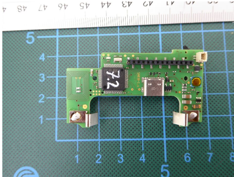
M420 PRO, PCB, front view
