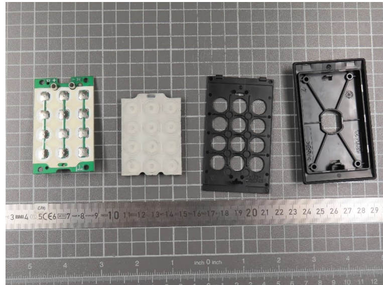
TA03, housing opened, view 1
