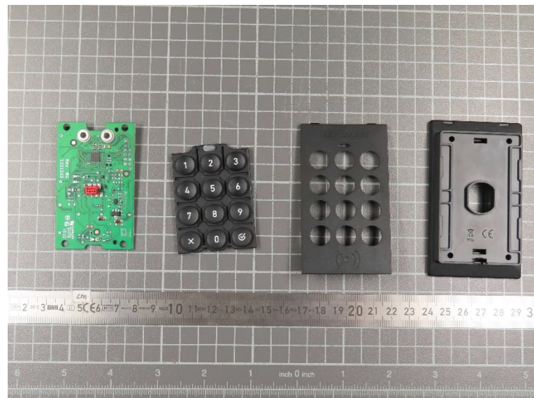
TA03 housing opened, view 2
