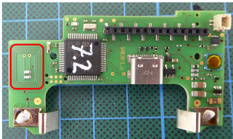
M420 PRO, passive RFID Antenna marked red
