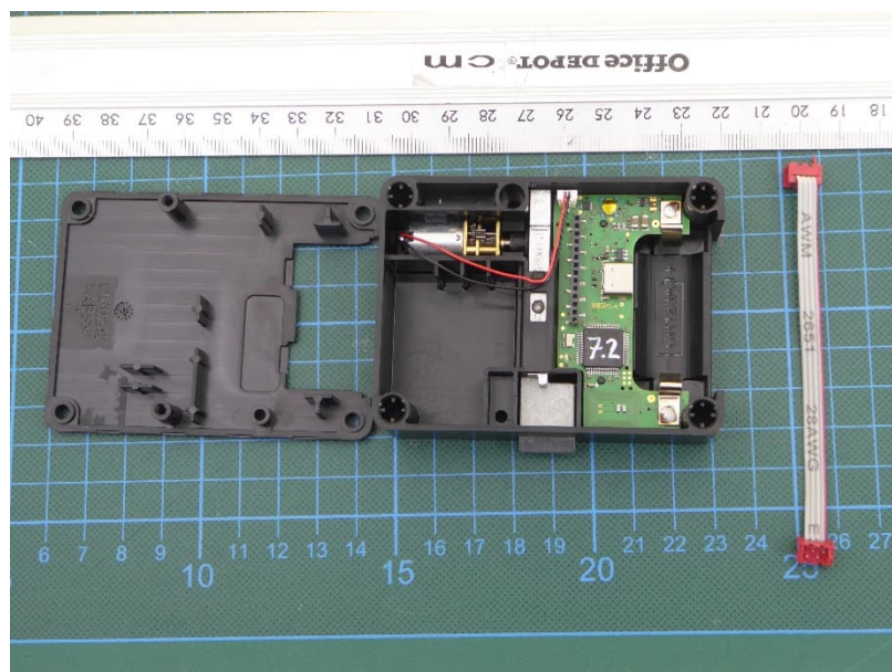
M420 PRO, housing opened, view 2
