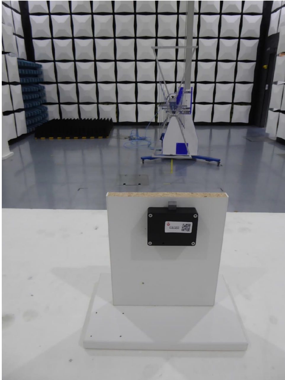
Test setup SAC Measurement of E-Field 30 MHz – 1000 MHz
