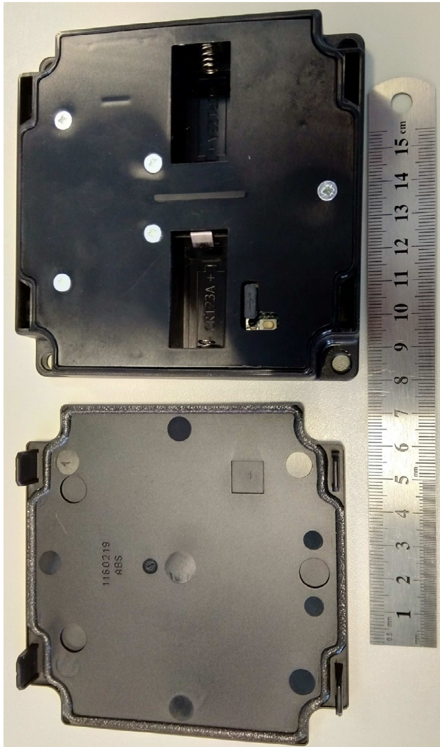
Bottom Side with cover – M610 TA pro
